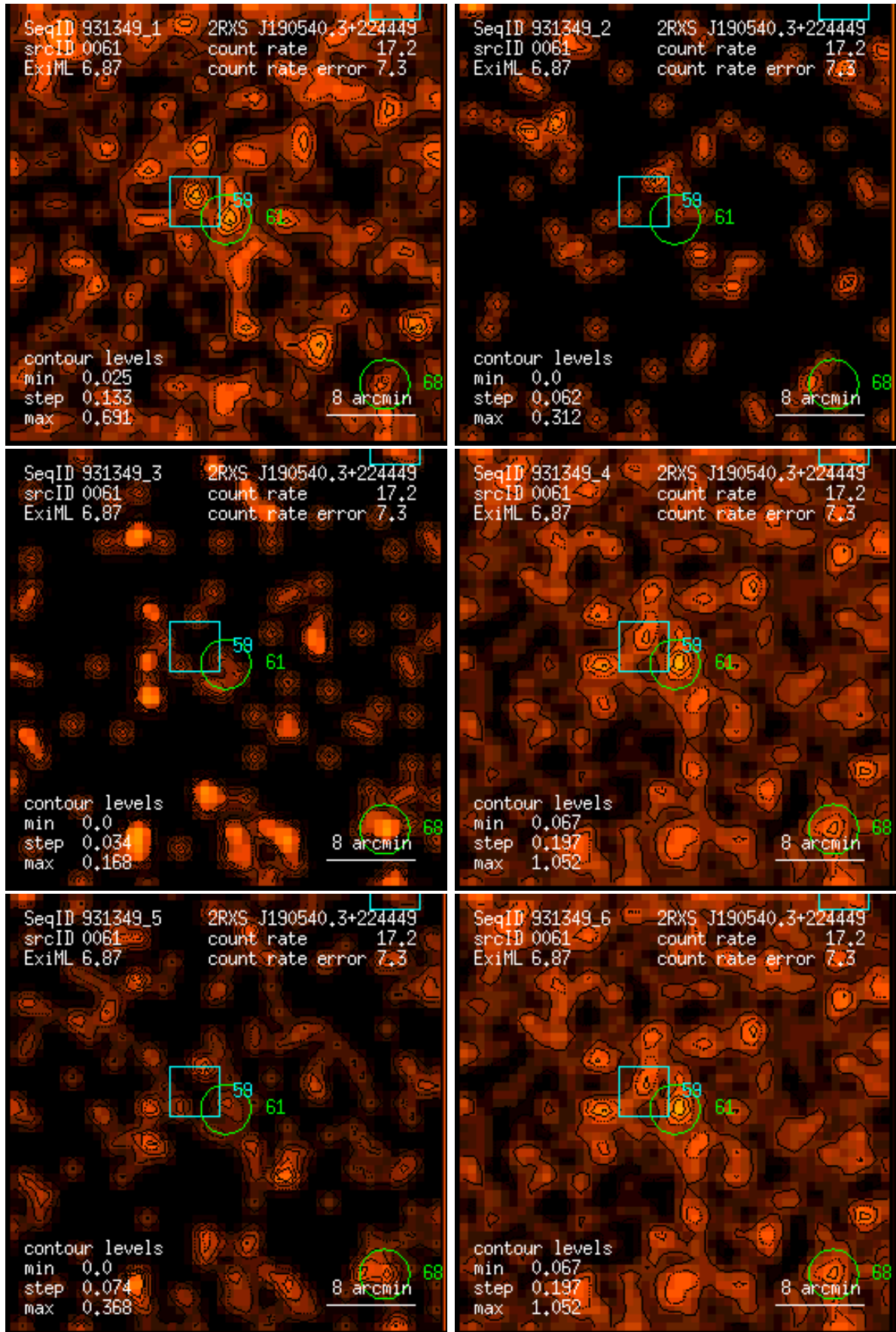
Figure 61: RASS 931349: detection 0061: band rate images, Gaussian filter: (1) PSPC channels 11 – 41, (2) 52 – 90, (3) 91 – 201, (4) 11 – 235, (5) 52 – 201, (6) 11 – 201. Broad band rates in counts/ks. Band rate contour levels in counts/ks/arcmin 2 .
