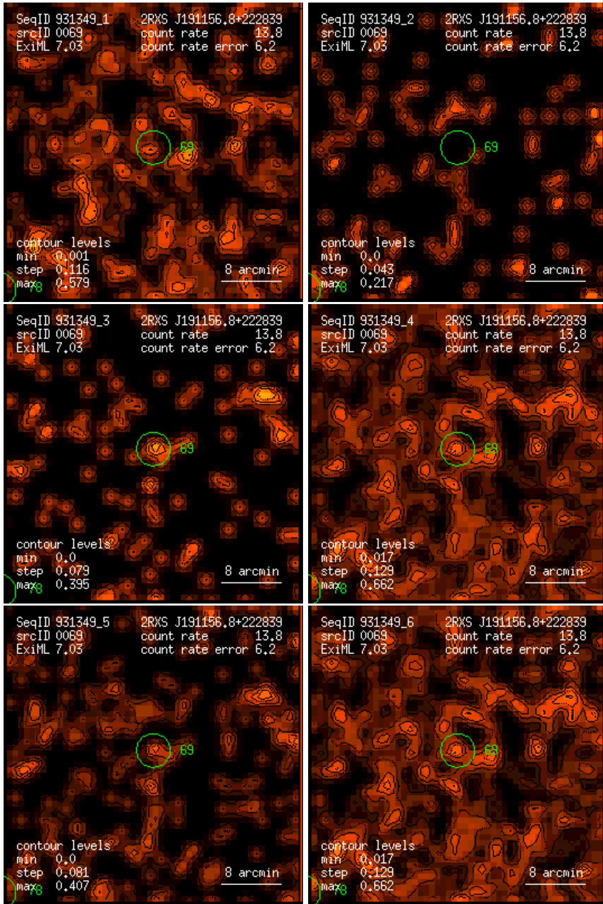
Figure 69: RASS 931349: detection 0069: band rate images, Gaussian filter: (1) PSPC channels 11 – 41, (2) 52 – 90, (3) 91 – 201, (4) 11 – 235, (5) 52 – 201, (6) 11 – 201. Broad band rates in counts/ks. Band rate contour levels in counts/ks/arcmin 2 .
