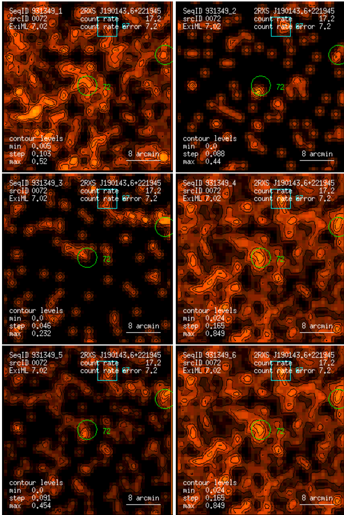
Figure 72: RASS 931349: detection 0072: band rate images, Gaussian filter: (1) PSPC channels 11 – 41, (2) 52 – 90, (3) 91 – 201, (4) 11 – 235, (5) 52 – 201, (6) 11 – 201. Broad band rates in counts/ks. Band rate contour levels in counts/ks/arcmin 2 .
