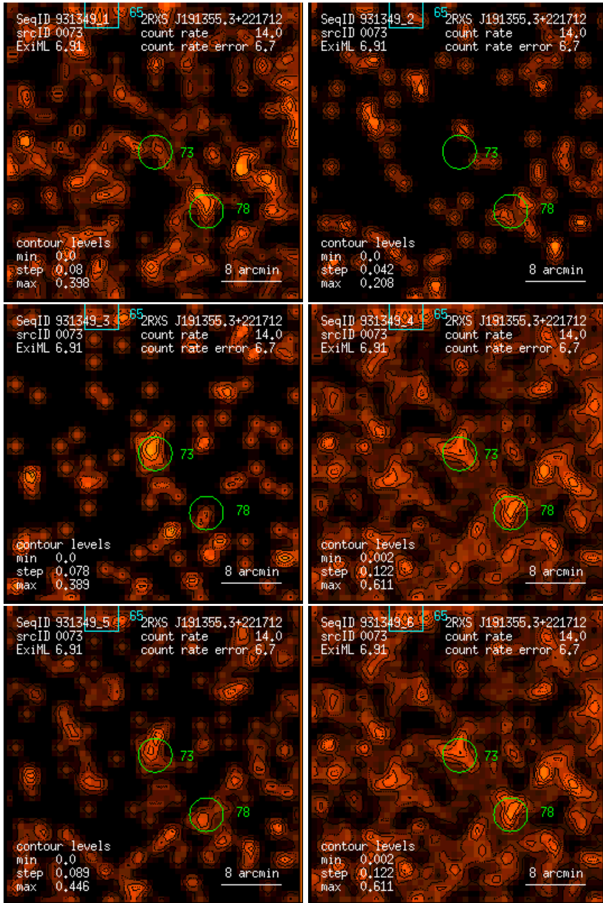
Figure 73: RASS 931349: detection 0073: band rate images, Gaussian filter: (1) PSPC channels 11 – 41, (2) 52 – 90, (3) 91 – 201, (4) 11 – 235, (5) 52 – 201, (6) 11 – 201. Broad band rates in counts/ks. Band rate contour levels in counts/ks/arcmin 2 .
