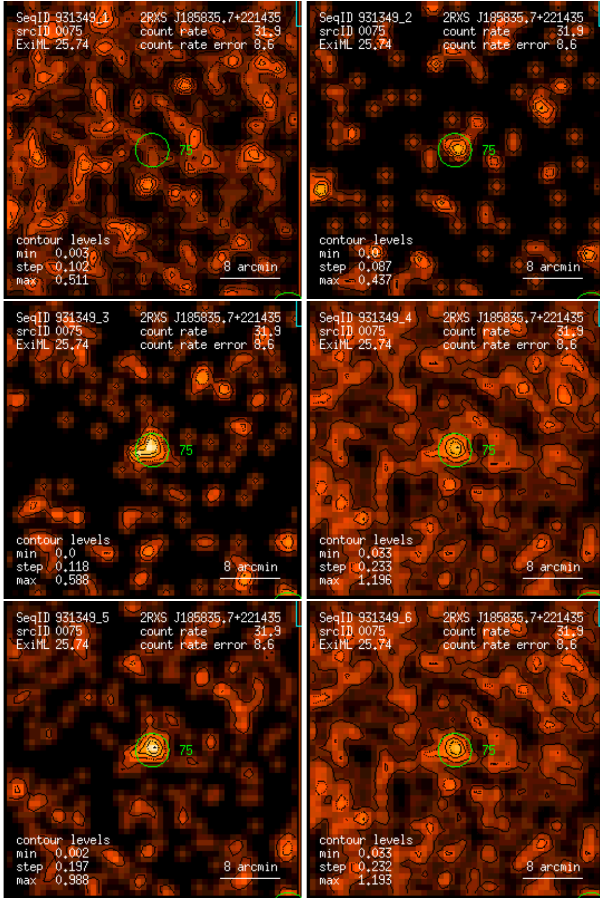
Figure 75: RASS 931349: detection 0075: band rate images, Gaussian filter: (1) PSPC channels 11 – 41, (2) 52 – 90, (3) 91 – 201, (4) 11 – 235, (5) 52 – 201, (6) 11 – 201. Broad band rates in counts/ks. Band rate contour levels in counts/ks/arcmin 2 .
