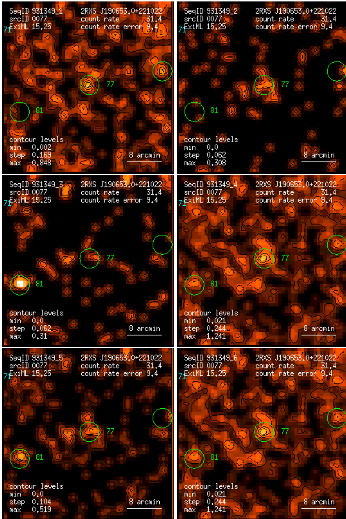
Figure 77: RASS 931349: detection 0077: band rate images, Gaussian filter: (1) PSPC channels 11 – 41, (2) 52 – 90, (3) 91 – 201, (4) 11 – 235, (5) 52 – 201, (6) 11 – 201. Broad band rates in counts/ks. Band rate contour levels in counts/ks/arcmin 2 .
