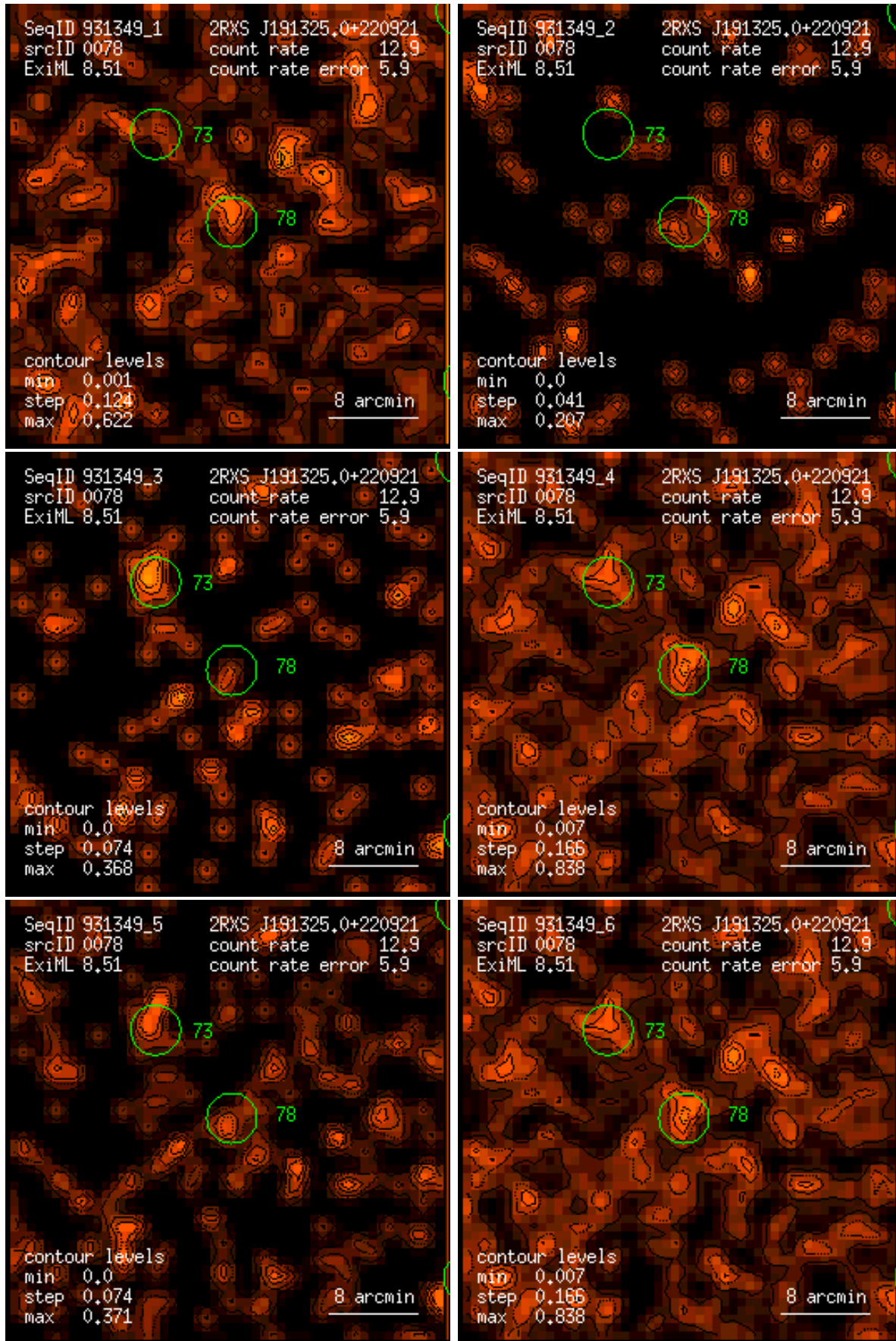
Figure 78: RASS 931349: detection 0078: band rate images, Gaussian filter: (1) PSPC channels 11 – 41, (2) 52 – 90, (3) 91 – 201, (4) 11 – 235, (5) 52 – 201, (6) 11 – 201. Broad band rates in counts/ks. Band rate contour levels in counts/ks/arcmin 2 .
