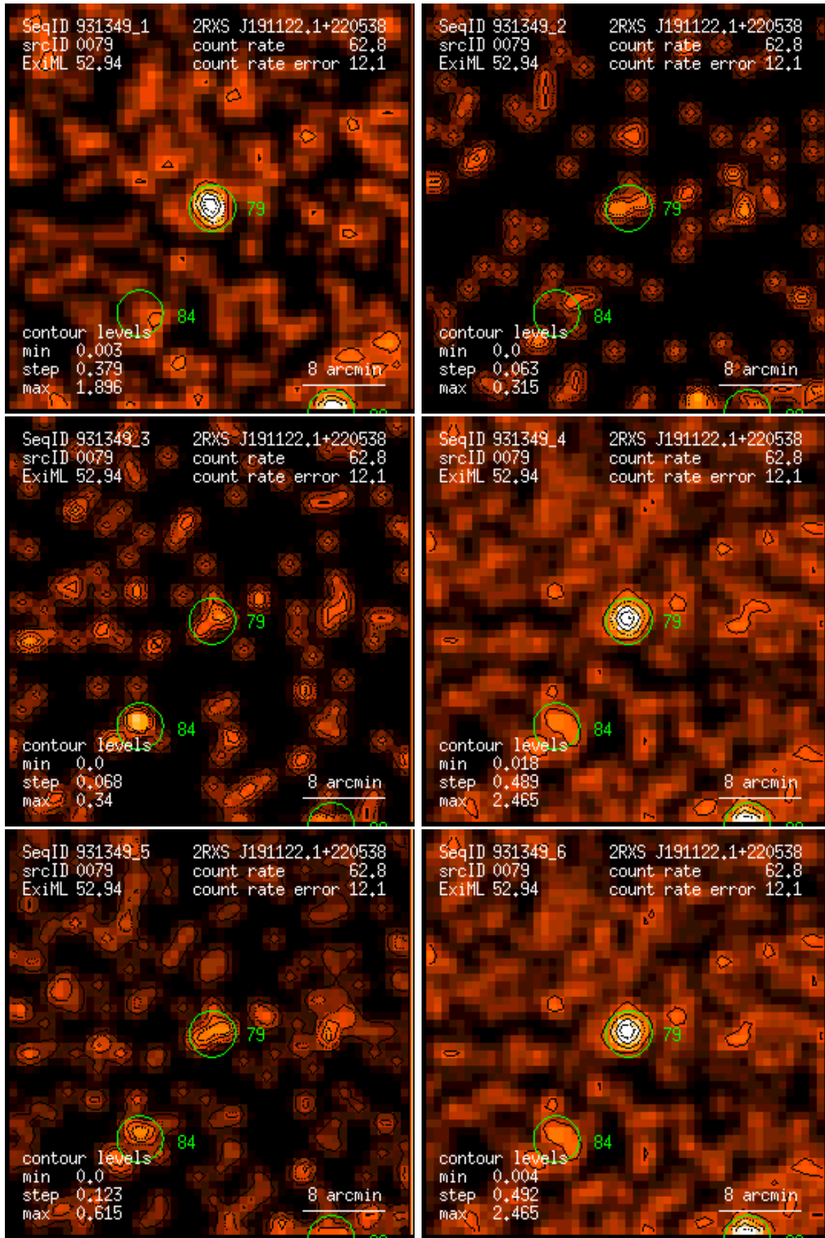
Figure 79: RASS 931349: detection 0079: band rate images, Gaussian filter: (1) PSPC channels 11 – 41, (2) 52 – 90, (3) 91 – 201, (4) 11 – 235, (5) 52 – 201, (6) 11 – 201. Broad band rates in counts/ks. Band rate contour levels in counts/ks/arcmin 2 .
