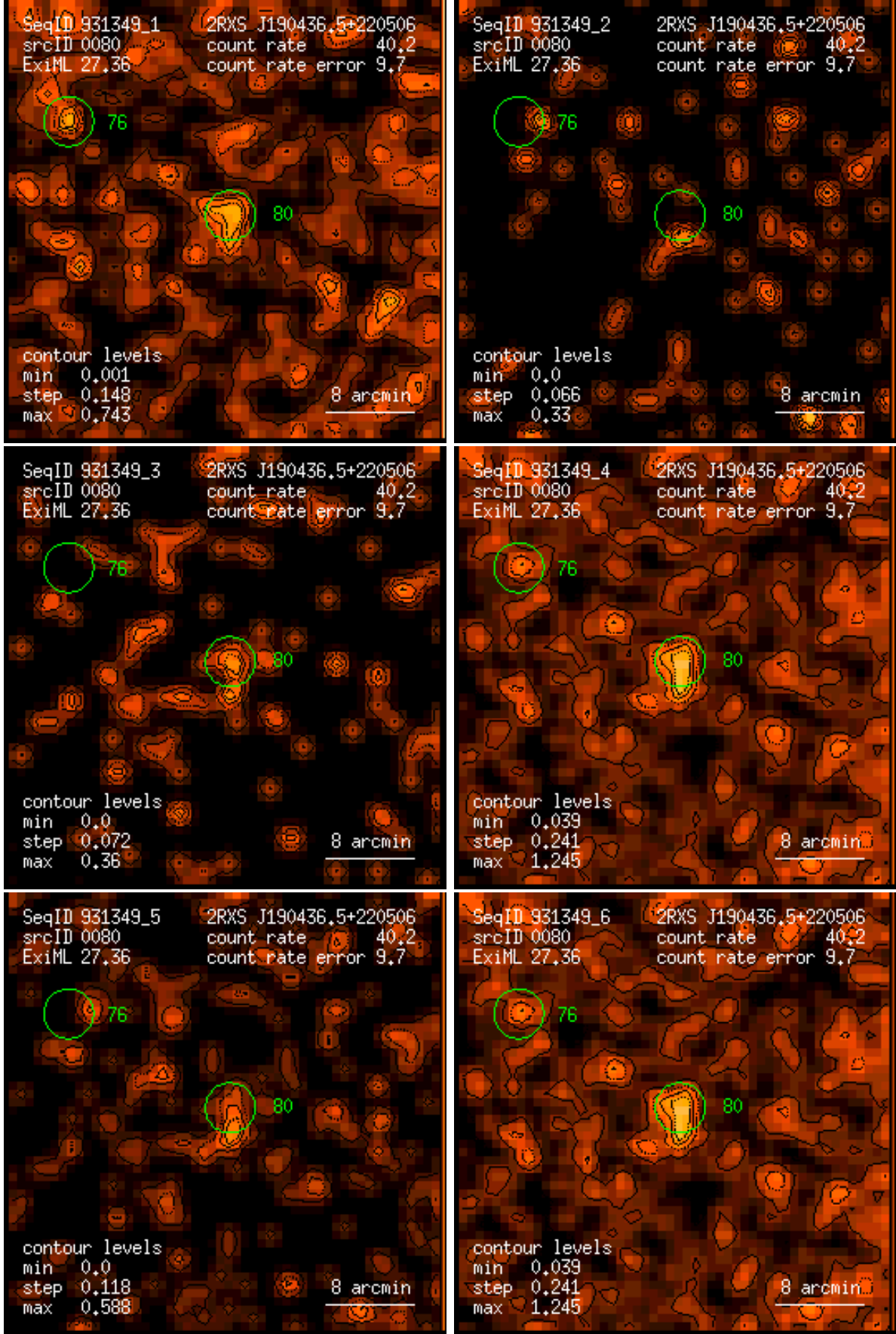
Figure 80: RASS 931349: detection 0080: band rate images, Gaussian filter: (1) PSPC channels 11 – 41, (2) 52 – 90, (3) 91 – 201, (4) 11 – 235, (5) 52 – 201, (6) 11 – 201. Broad band rates in counts/ks. Band rate contour levels in counts/ks/arcmin 2 .
