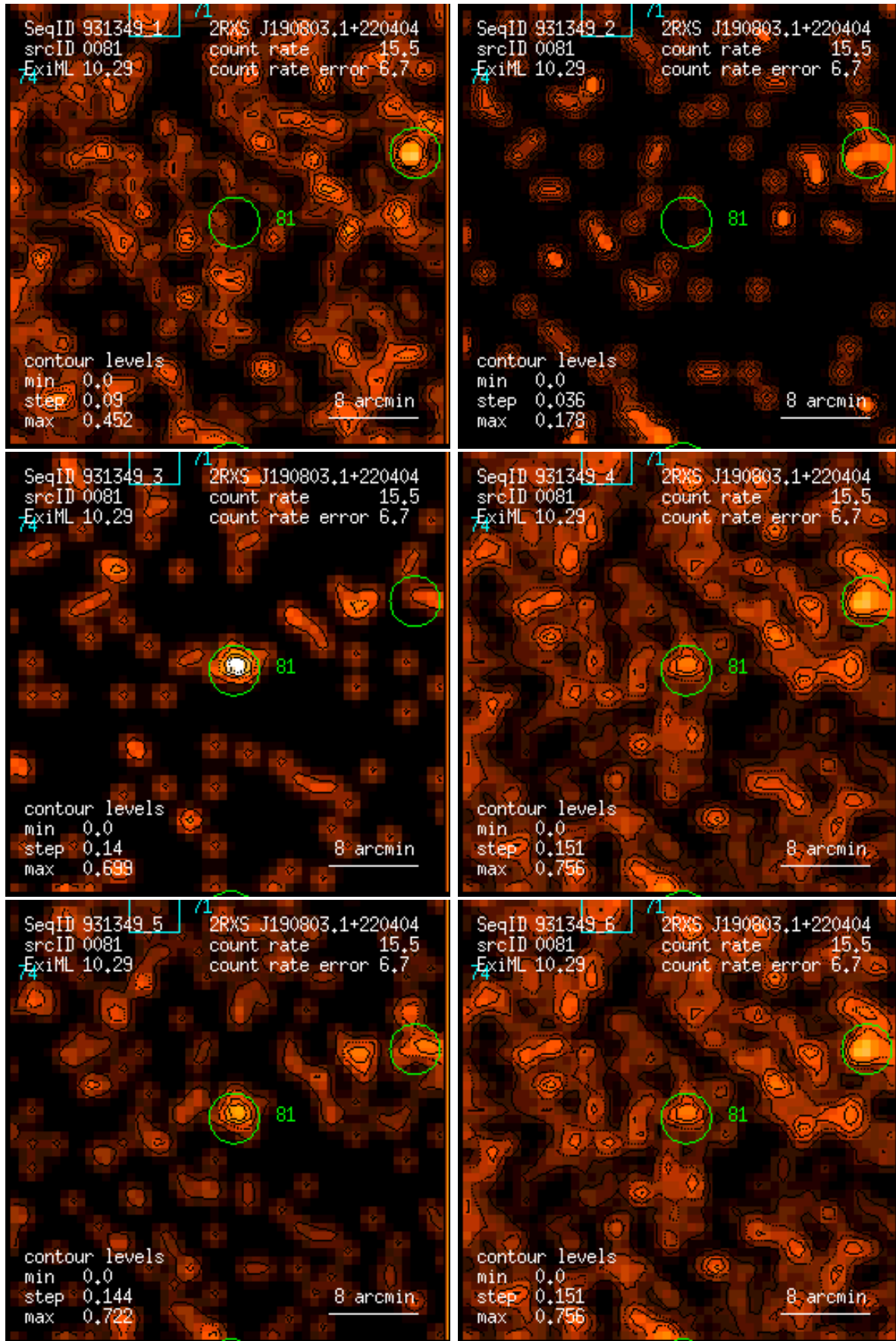
Figure 81: RASS 931349: detection 0081: band rate images, Gaussian filter: (1) PSPC channels 11 – 41, (2) 52 – 90, (3) 91 – 201, (4) 11 – 235, (5) 52 – 201, (6) 11 – 201. Broad band rates in counts/ks. Band rate contour levels in counts/ks/arcmin 2 .
