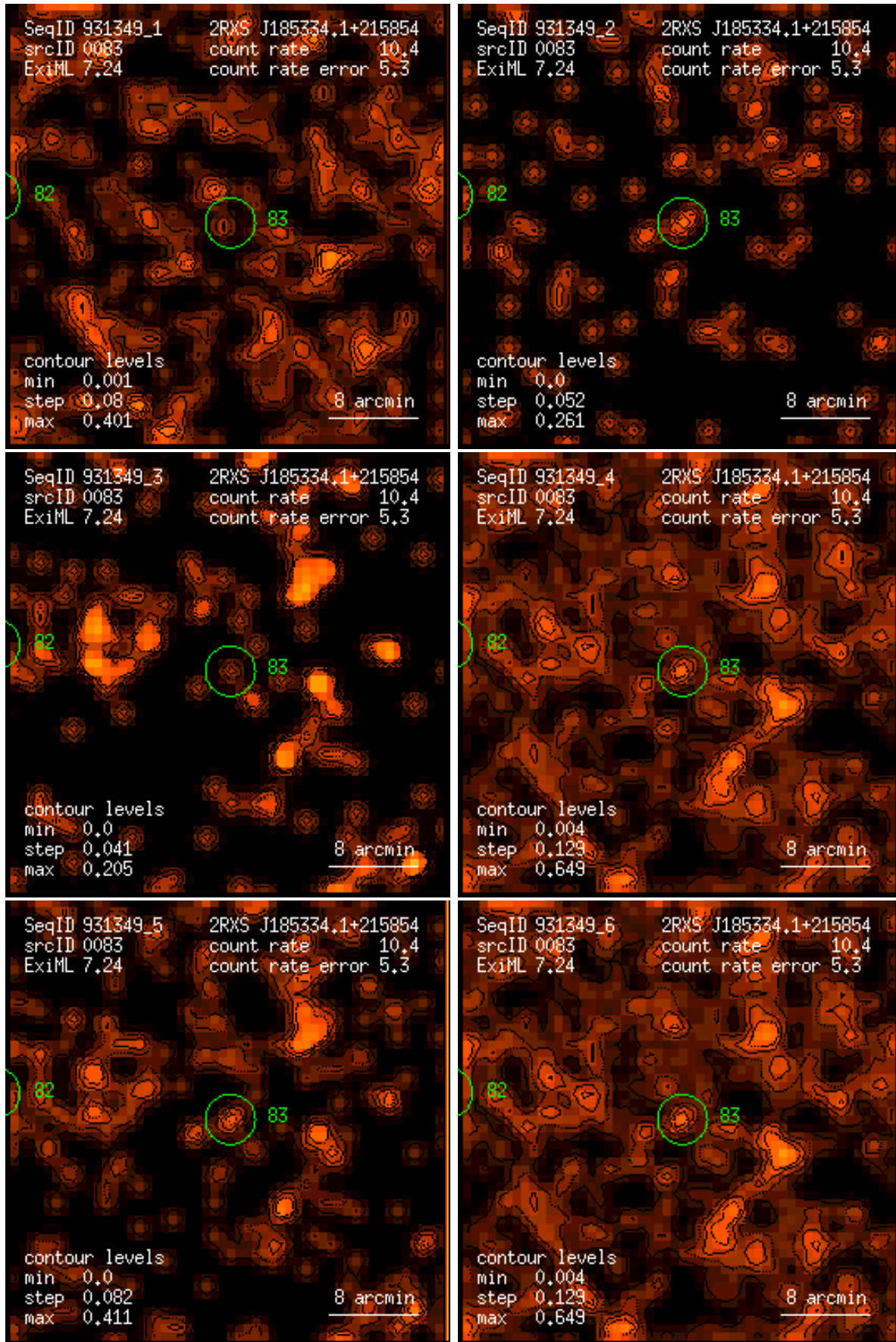
Figure 83: RASS 931349: detection 0083: band rate images, Gaussian filter: (1) PSPC channels 11 – 41, (2) 52 – 90, (3) 91 – 201, (4) 11 – 235, (5) 52 – 201, (6) 11 – 201. Broad band rates in counts/ks. Band rate contour levels in counts/ks/arcmin 2 .
