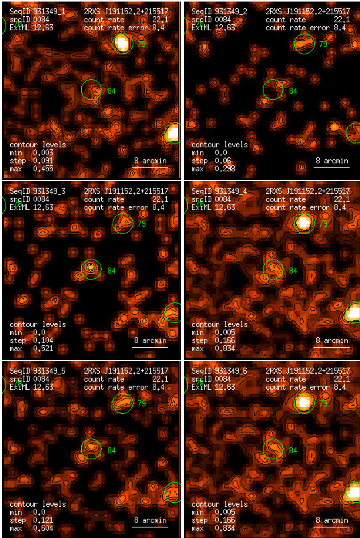
Figure 84: RASS 931349: detection 0084: band rate images, Gaussian filter: (1) PSPC channels 11 – 41, (2) 52 – 90, (3) 91 – 201, (4) 11 – 235, (5) 52 – 201, (6) 11 – 201. Broad band rates in counts/ks. Band rate contour levels in counts/ks/arcmin 2 .
