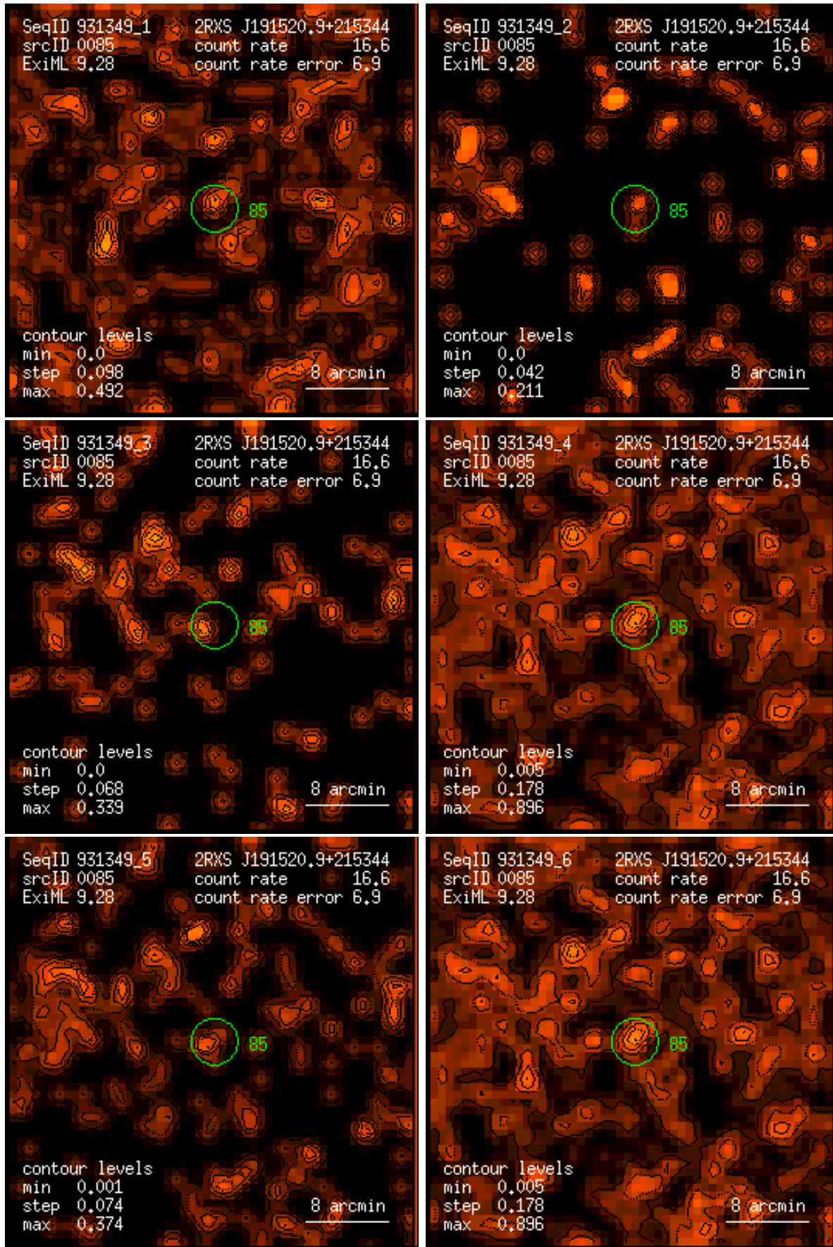
Figure 85: RASS 931349: detection 0085: band rate images, Gaussian filter: (1) PSPC channels 11 – 41, (2) 52 – 90, (3) 91 – 201, (4) 11 – 235, (5) 52 – 201, (6) 11 – 201. Broad band rates in counts/ks. Band rate contour levels in counts/ks/arcmin 2 .
