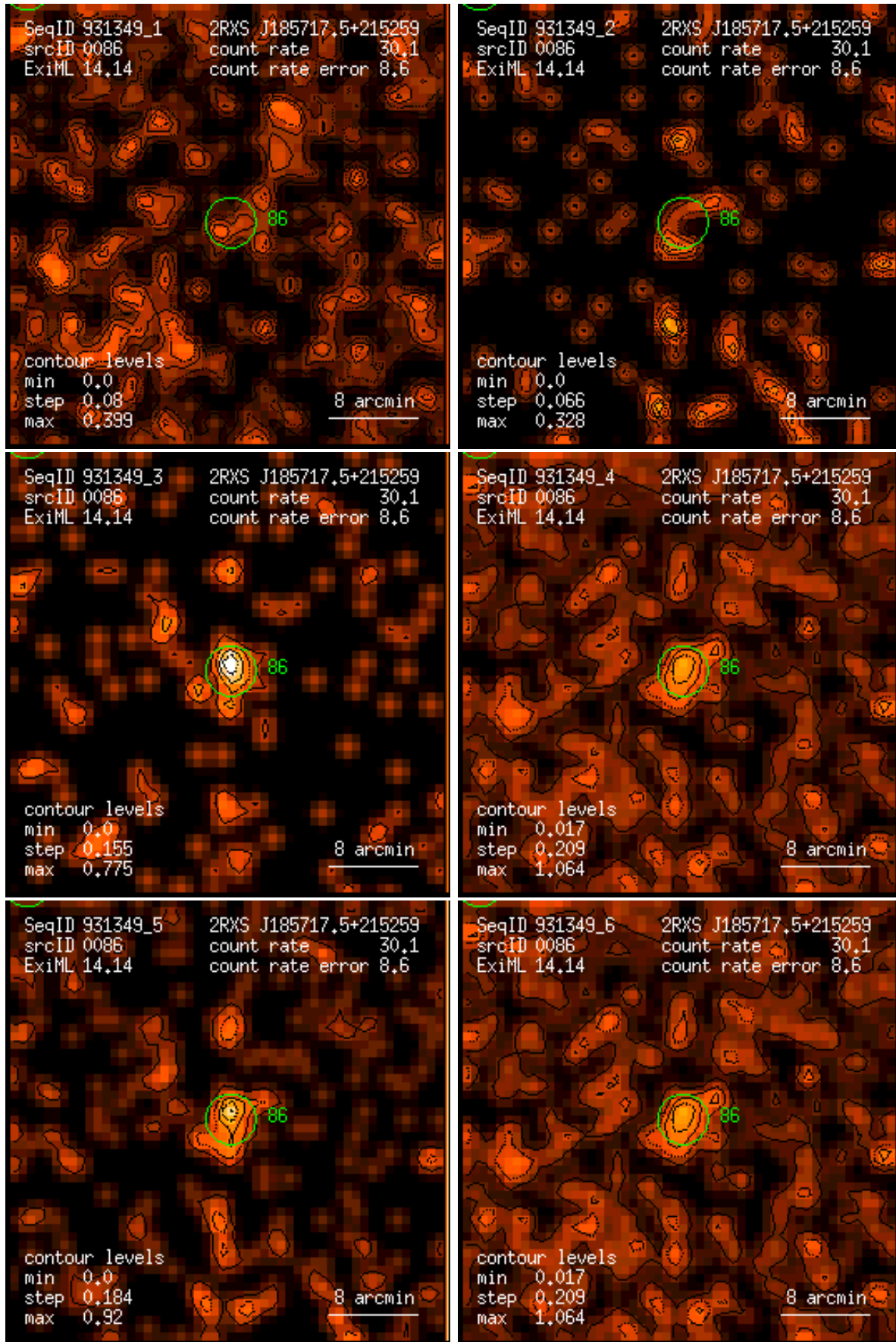
Figure 86: RASS 931349: detection 0086: band rate images, Gaussian filter: (1) PSPC channels 11 – 41, (2) 52 – 90, (3) 91 – 201, (4) 11 – 235, (5) 52 – 201, (6) 11 – 201. Broad band rates in counts/ks. Band rate contour levels in counts/ks/arcmin 2 .
