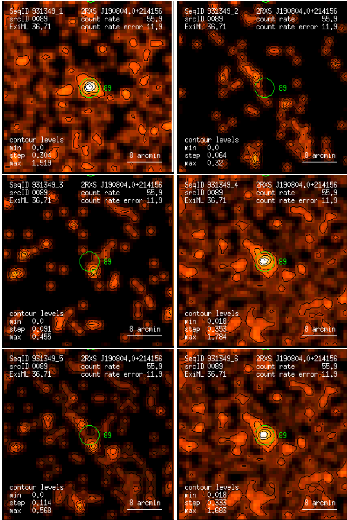
Figure 89: RASS 931349: detection 0089: band rate images, Gaussian filter: (1) PSPC channels 11 – 41, (2) 52 – 90, (3) 91 – 201, (4) 11 – 235, (5) 52 – 201, (6) 11 – 201. Broad band rates in counts/ks. Band rate contour levels in counts/ks/arcmin 2 .
