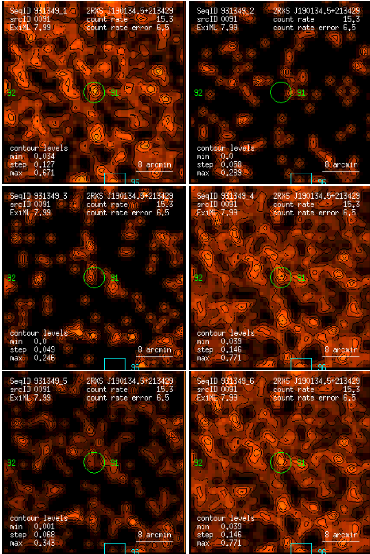
Figure 91: RASS 931349: detection 0091: band rate images, Gaussian filter: (1) PSPC channels 11 – 41, (2) 52 – 90, (3) 91 – 201, (4) 11 – 235, (5) 52 – 201, (6) 11 – 201. Broad band rates in counts/ks. Band rate contour levels in counts/ks/arcmin 2 .
