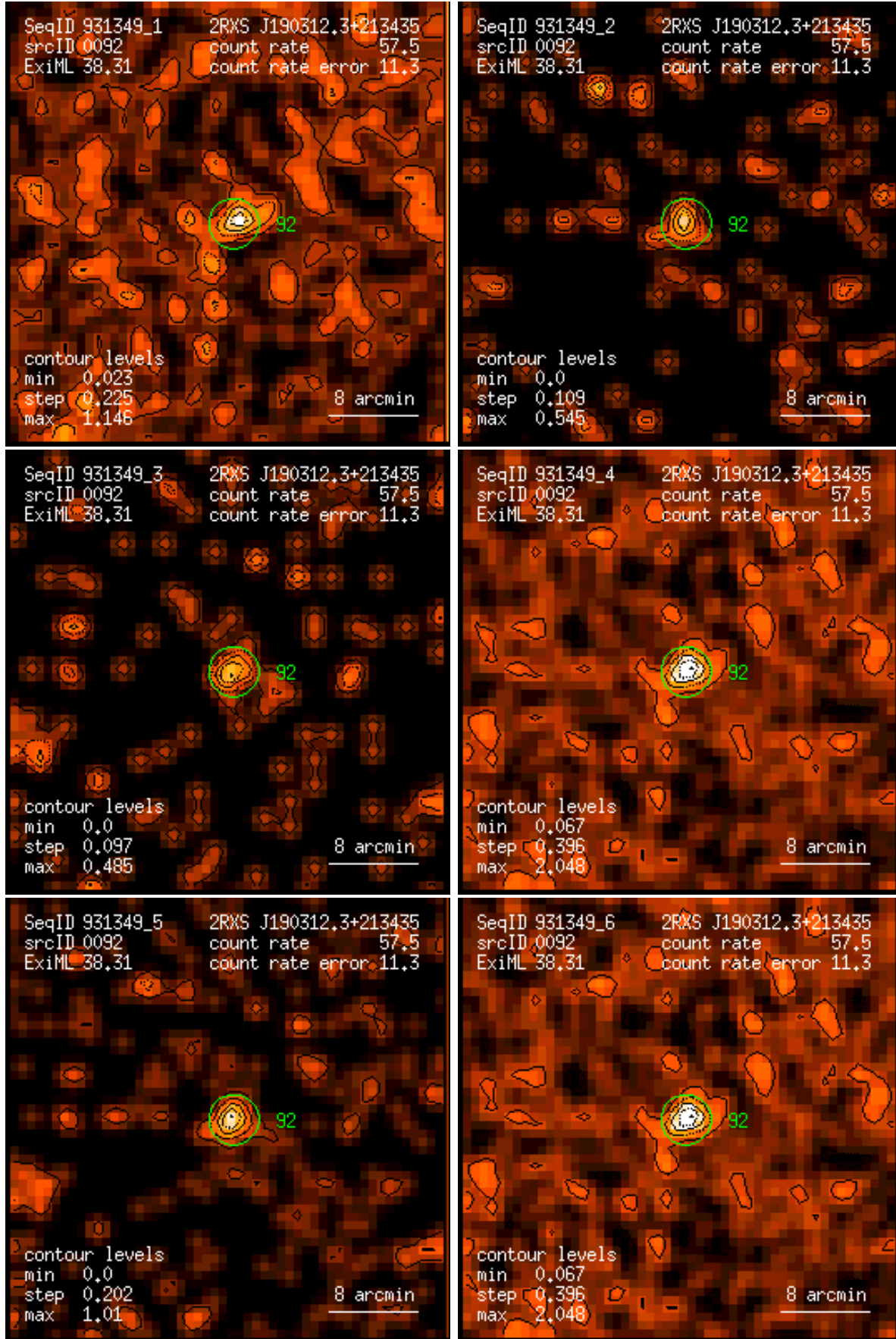
Figure 92: RASS 931349: detection 0092: band rate images, Gaussian filter: (1) PSPC channels 11 – 41, (2) 52 – 90, (3) 91 – 201, (4) 11 – 235, (5) 52 – 201, (6) 11 – 201. Broad band rates in counts/ks. Band rate contour levels in counts/ks/arcmin 2 .
