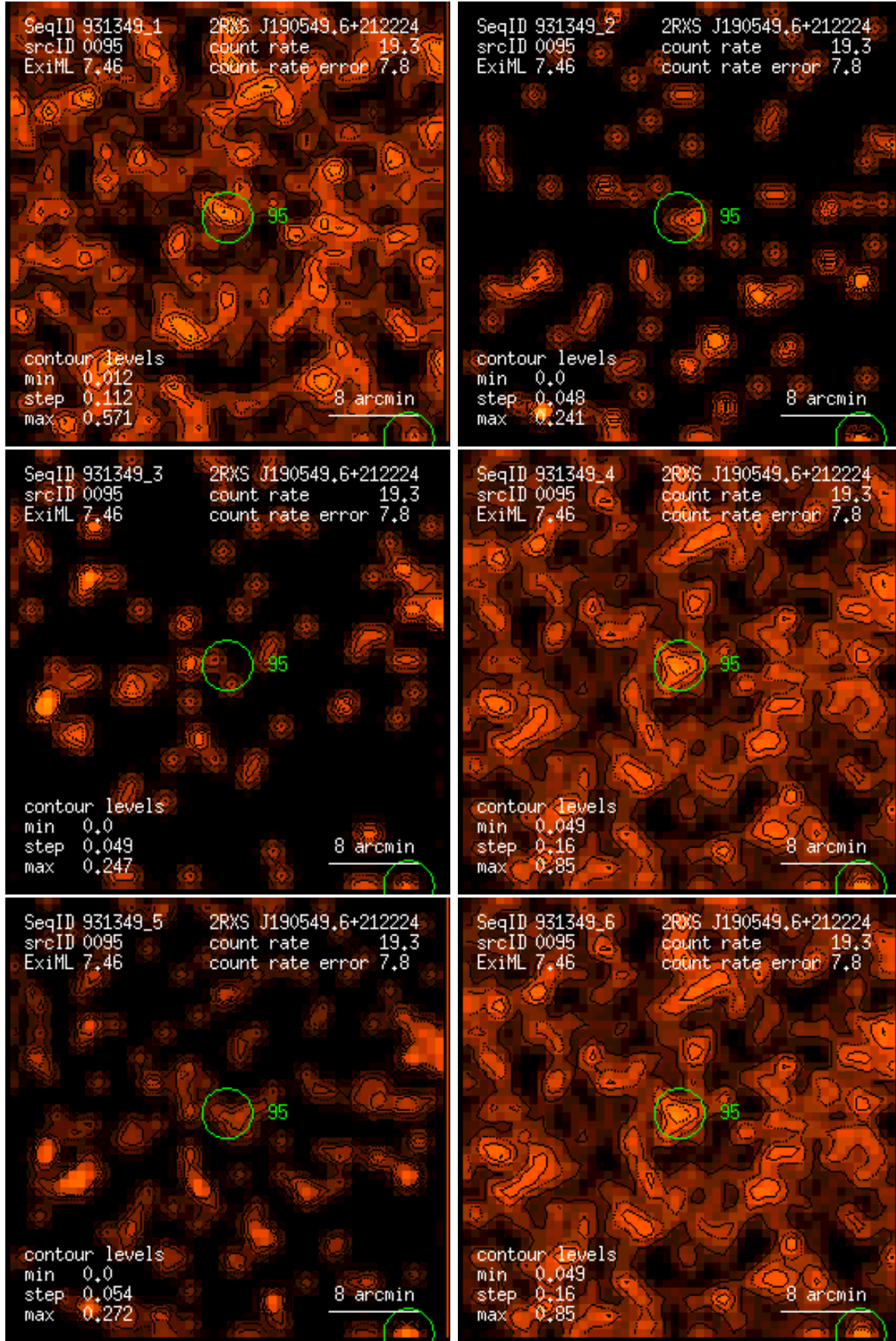
Figure 95: RASS 931349: detection 0095: band rate images, Gaussian filter: (1) PSPC channels 11 – 41, (2) 52 – 90, (3) 91 – 201, (4) 11 – 235, (5) 52 – 201, (6) 11 – 201. Broad band rates in counts/ks. Band rate contour levels in counts/ks/arcmin 2 .
