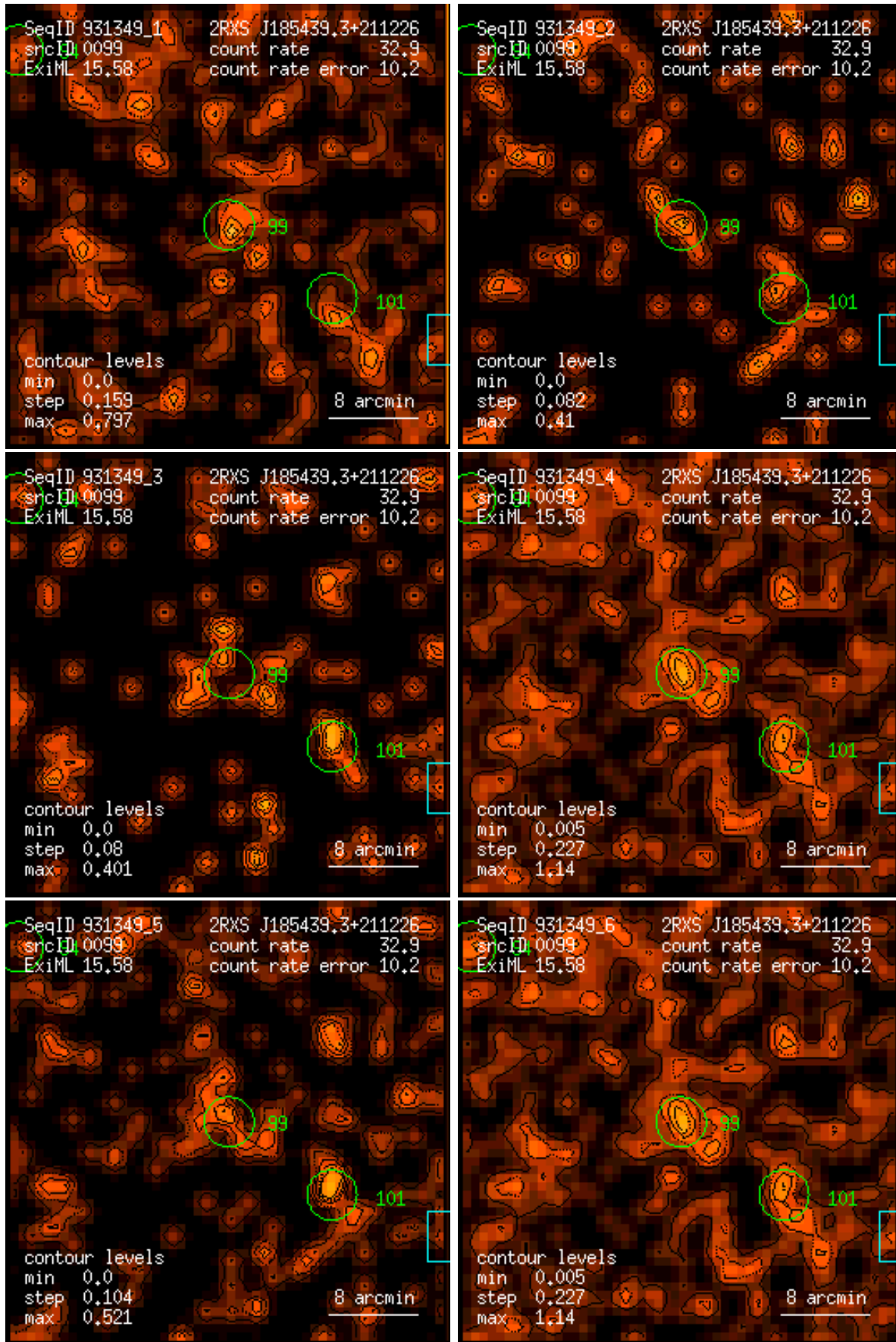
Figure 99: RASS 931349: detection 0099: band rate images, Gaussian filter: (1) PSPC channels 11 – 41, (2) 52 – 90, (3) 91 – 201, (4) 11 – 235, (5) 52 – 201, (6) 11 – 201. Broad band rates in counts/ks. Band rate contour levels in counts/ks/arcmin 2 .
