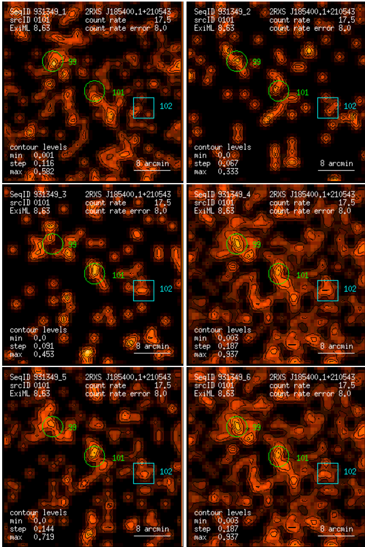
Figure 101: RASS 931349: detection 0101: band rate images, Gaussian filter: (1) PSPC channels 11 – 41, (2) 52 – 90, (3) 91 – 201, (4) 11 – 235, (5) 52 – 201, (6) 11 – 201. Broad band rates in counts/ks. Band rate contour levels in counts/ks/arcmin 2 .
