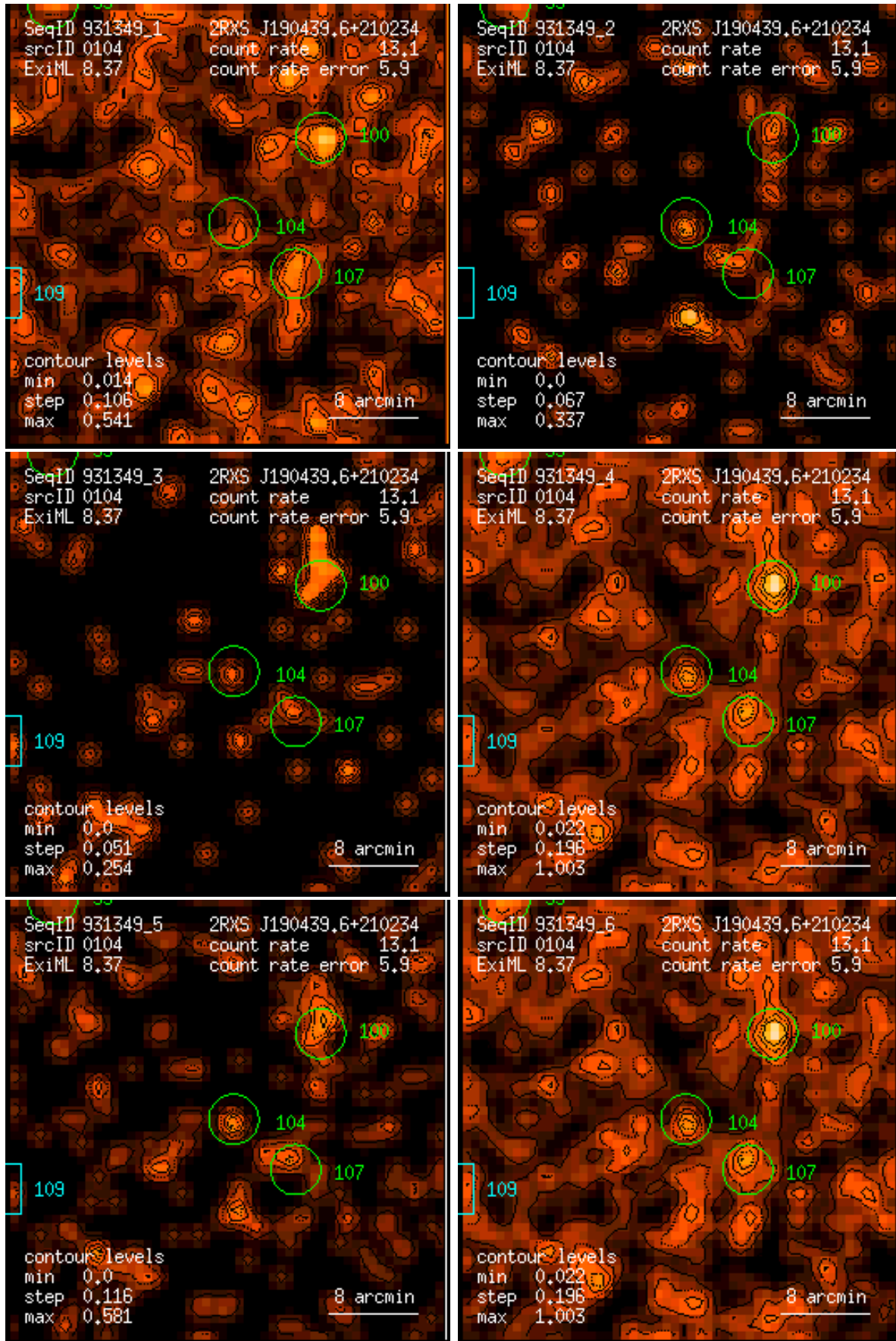
Figure 104: RASS 931349: detection 0104: band rate images, Gaussian filter: (1) PSPC channels 11 – 41, (2) 52 – 90, (3) 91 – 201, (4) 11 – 235, (5) 52 – 201, (6) 11 – 201. Broad band rates in counts/ks. Band rate contour levels in counts/ks/arcmin 2 .
