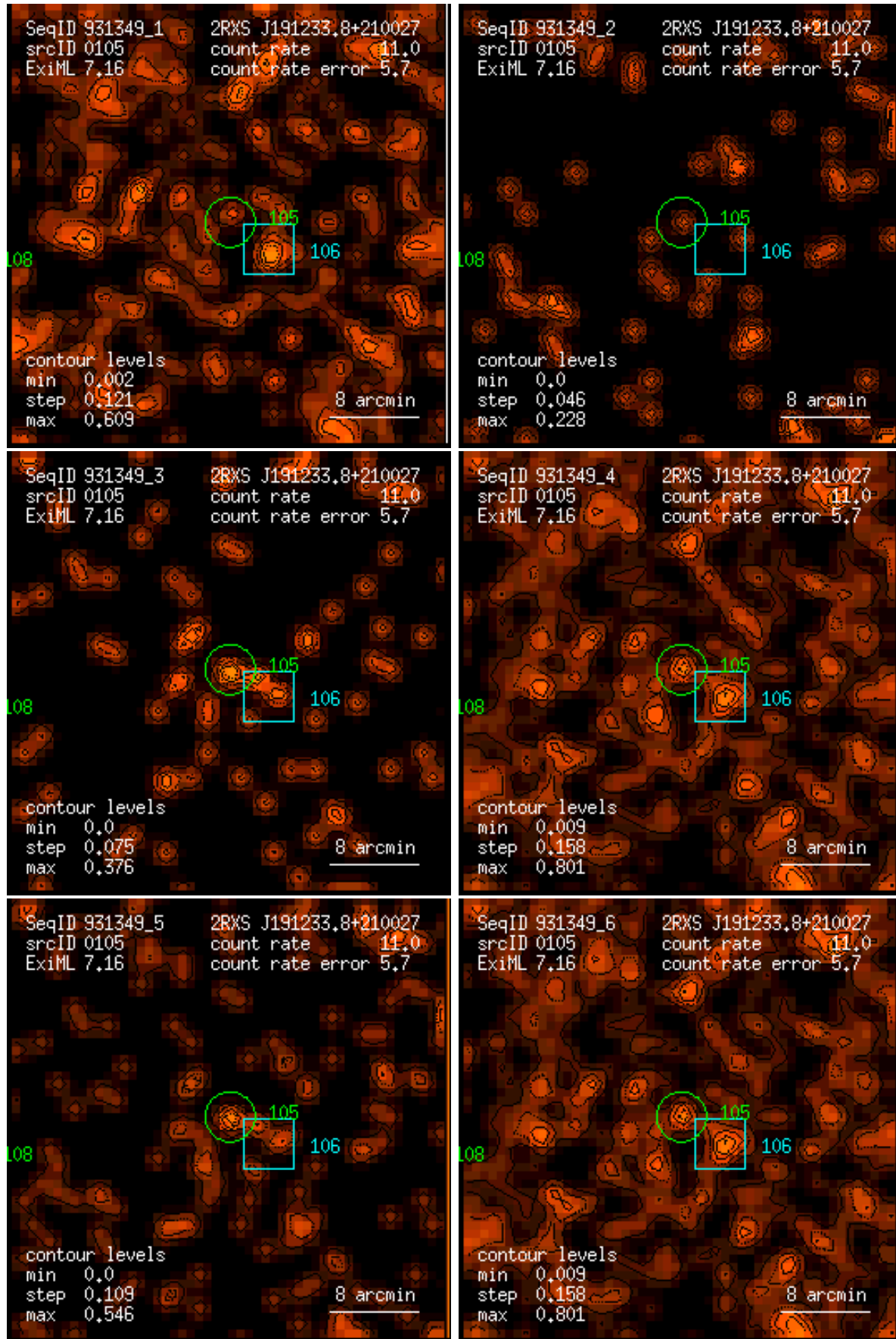
Figure 105: RASS 931349: detection 0105: band rate images, Gaussian filter: (1) PSPC channels 11 – 41, (2) 52 – 90, (3) 91 – 201, (4) 11 – 235, (5) 52 – 201, (6) 11 – 201. Broad band rates in counts/ks. Band rate contour levels in counts/ks/arcmin 2 .
