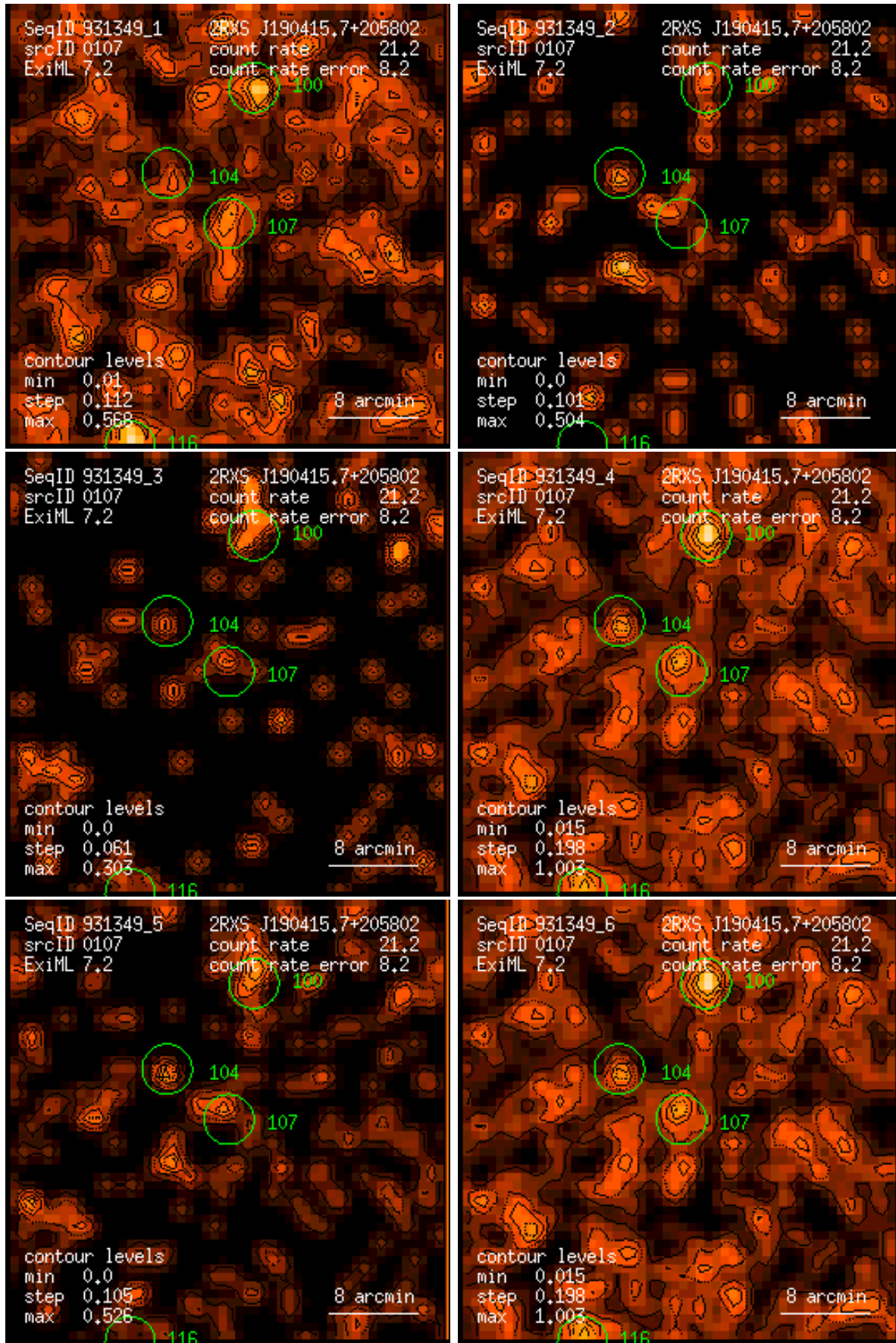
Figure 107: RASS 931349: detection 0107: band rate images, Gaussian filter: (1) PSPC channels 11 – 41, (2) 52 – 90, (3) 91 – 201, (4) 11 – 235, (5) 52 – 201, (6) 11 – 201. Broad band rates in counts/ks. Band rate contour levels in counts/ks/arcmin 2 .
