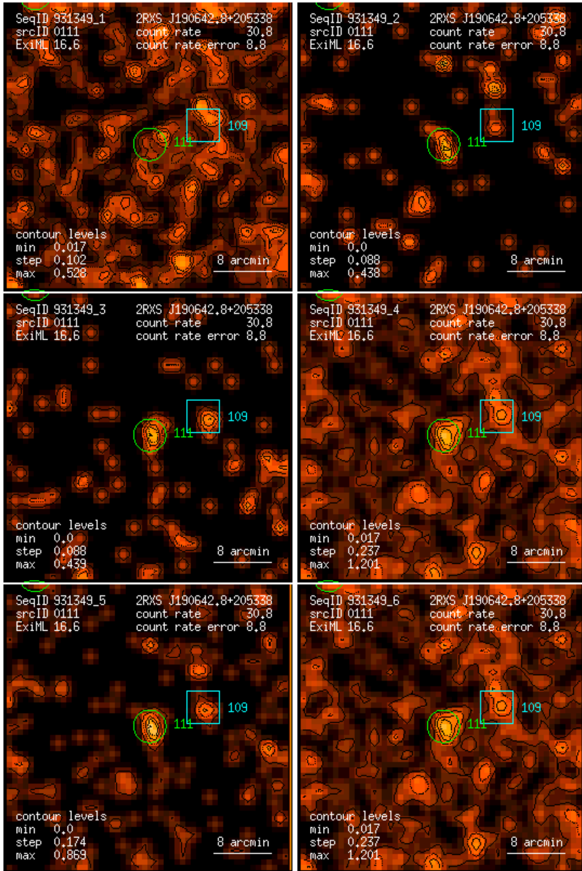
Figure 111: RASS 931349: detection 0111: band rate images, Gaussian filter: (1) PSPC channels 11 – 41, (2) 52 – 90, (3) 91 – 201, (4) 11 – 235, (5) 52 – 201, (6) 11 – 201. Broad band rates in counts/ks. Band rate contour levels in counts/ks/arcmin 2 .
