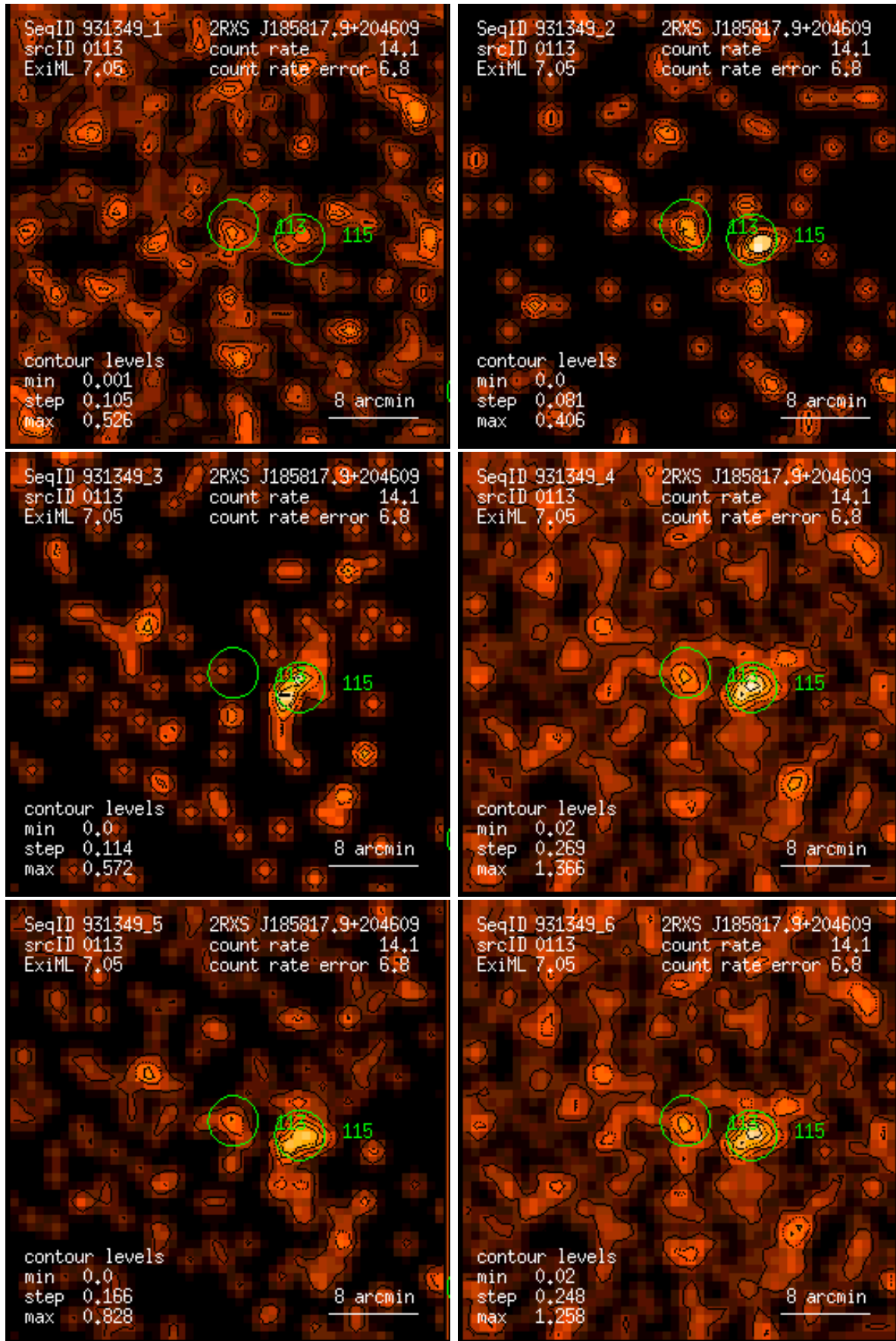
Figure 113: RASS 931349: detection 0113: band rate images, Gaussian filter: (1) PSPC channels 11 – 41, (2) 52 – 90, (3) 91 – 201, (4) 11 – 235, (5) 52 – 201, (6) 11 – 201. Broad band rates in counts/ks. Band rate contour levels in counts/ks/arcmin 2 .
