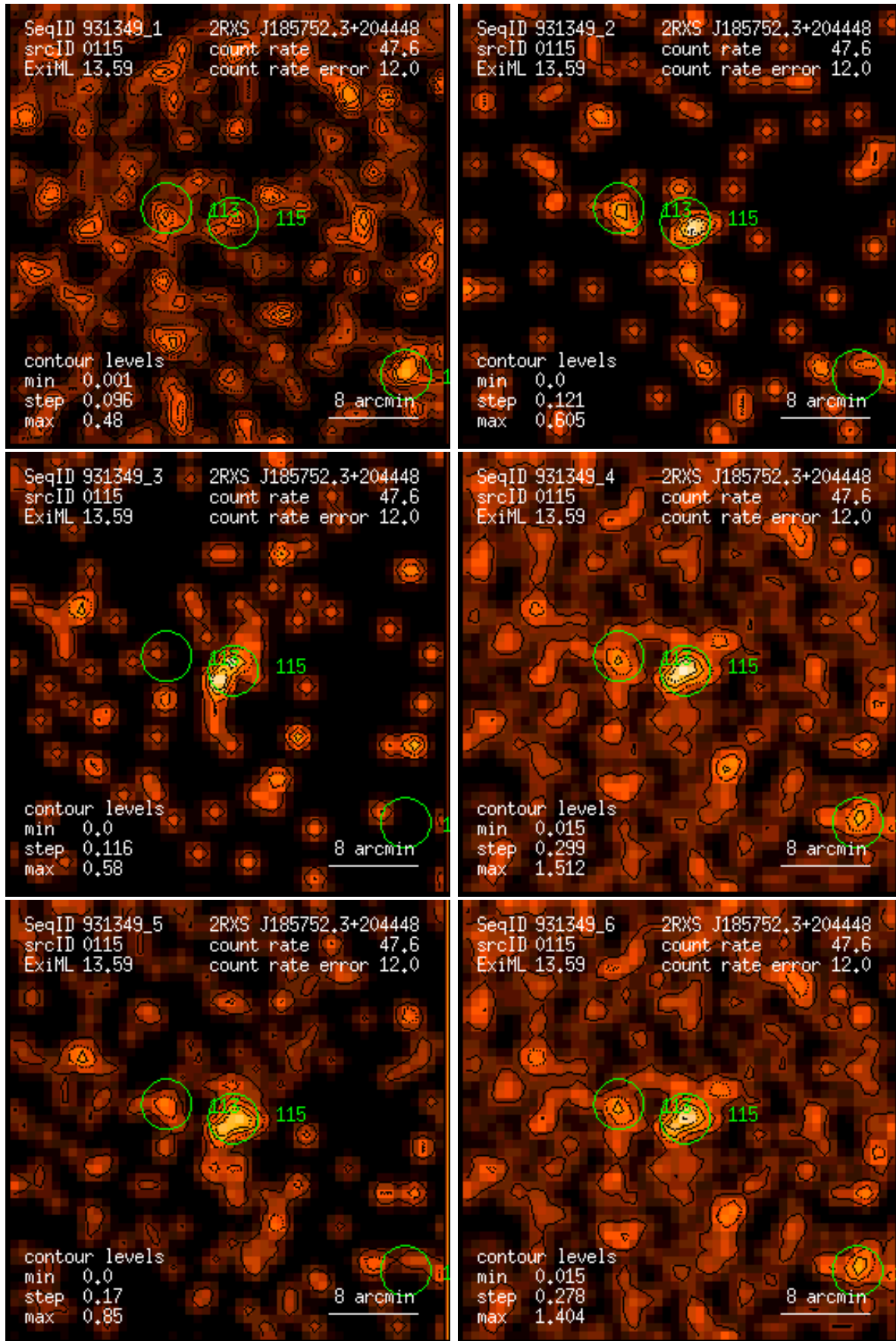
Figure 115: RASS 931349: detection 0115: band rate images, Gaussian filter: (1) PSPC channels 11 – 41, (2) 52 – 90, (3) 91 – 201, (4) 11 – 235, (5) 52 – 201, (6) 11 – 201. Broad band rates in counts/ks. Band rate contour levels in counts/ks/arcmin 2 .
