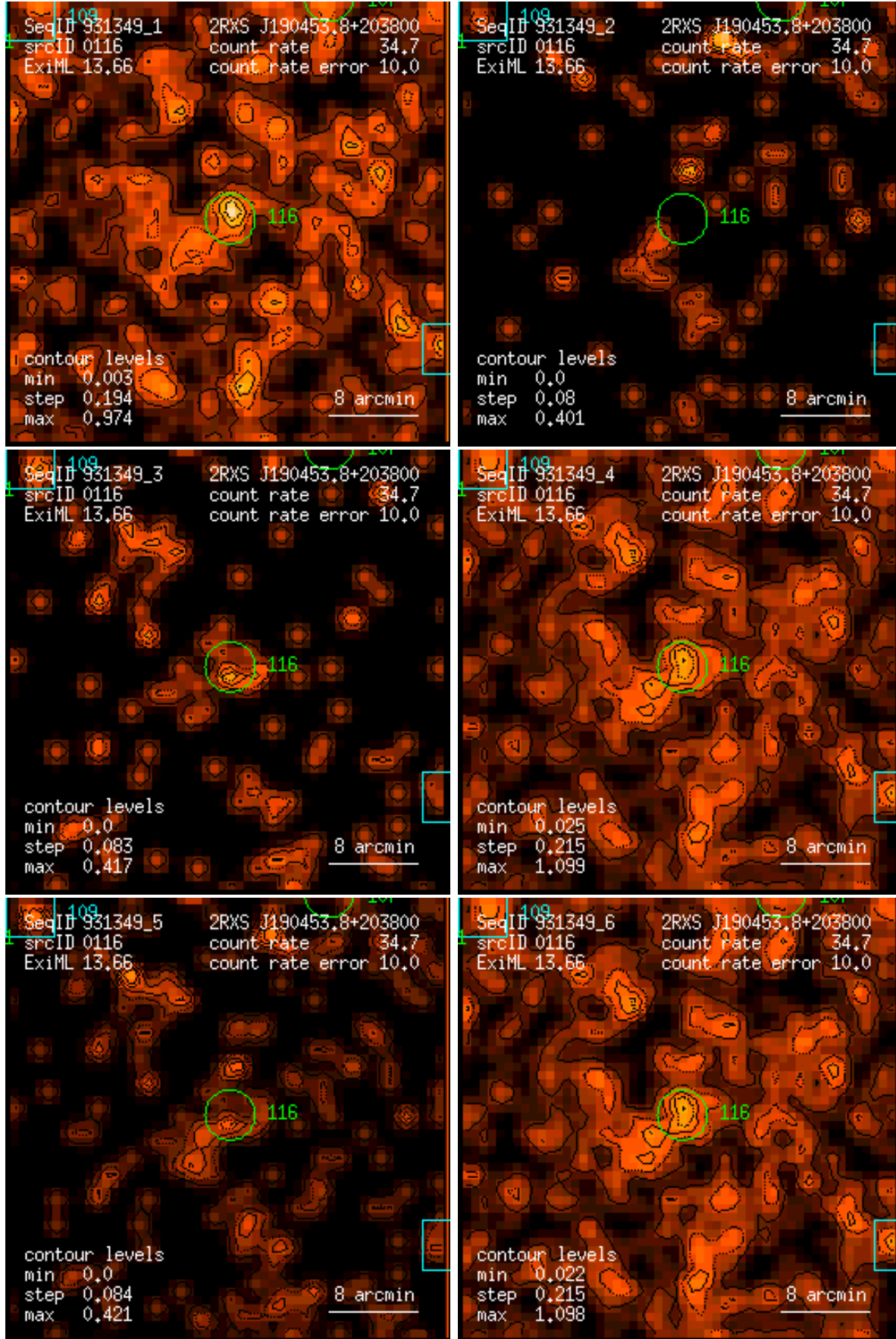
Figure 116: RASS 931349: detection 0116: band rate images, Gaussian filter: (1) PSPC channels 11 – 41, (2) 52 – 90, (3) 91 – 201, (4) 11 – 235, (5) 52 – 201, (6) 11 – 201. Broad band rates in counts/ks. Band rate contour levels in counts/ks/arcmin 2 .
