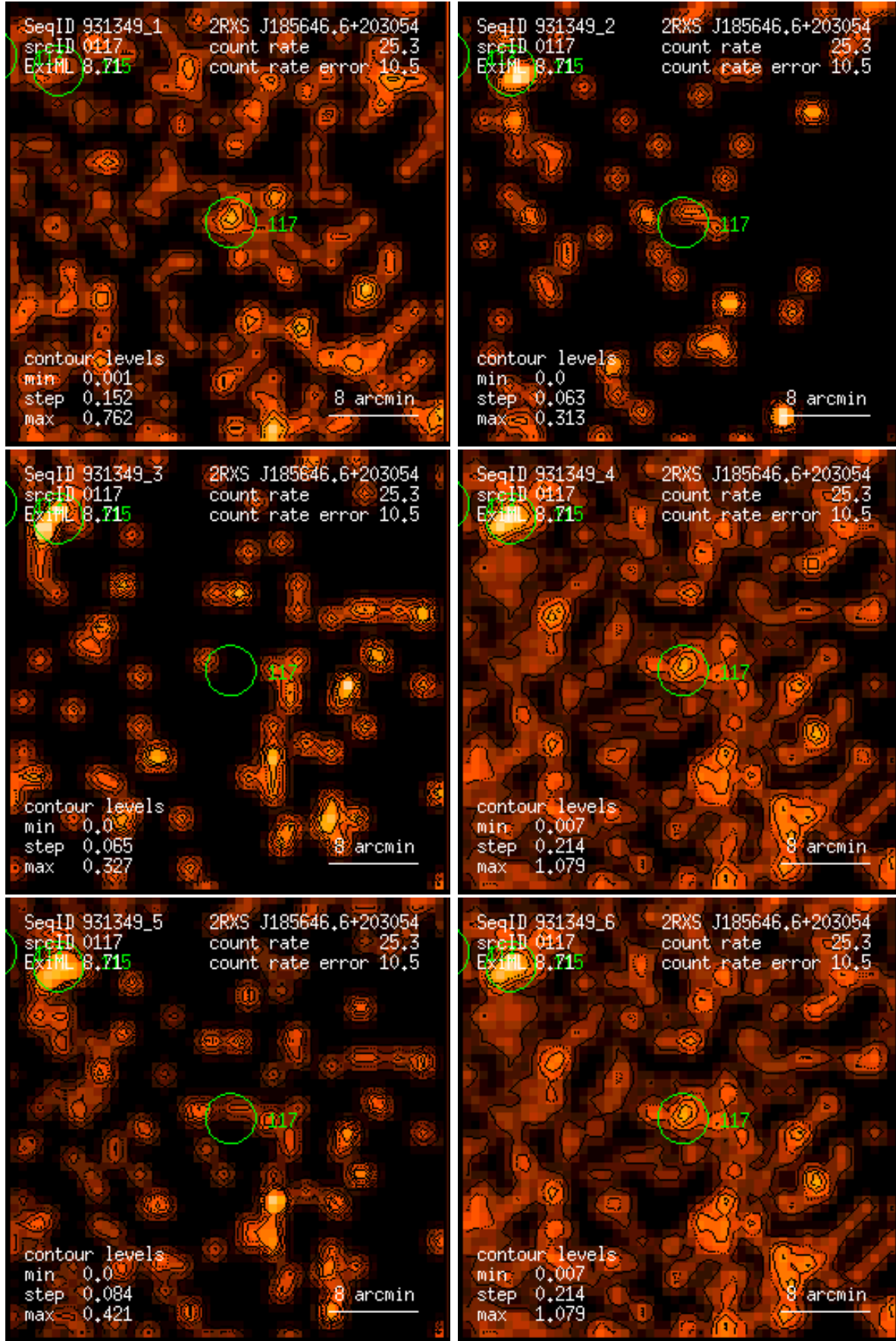
Figure 117: RASS 931349: detection 0117: band rate images, Gaussian filter: (1) PSPC channels 11 – 41, (2) 52 – 90, (3) 91 – 201, (4) 11 – 235, (5) 52 – 201, (6) 11 – 201. Broad band rates in counts/ks. Band rate contour levels in counts/ks/arcmin 2 .
