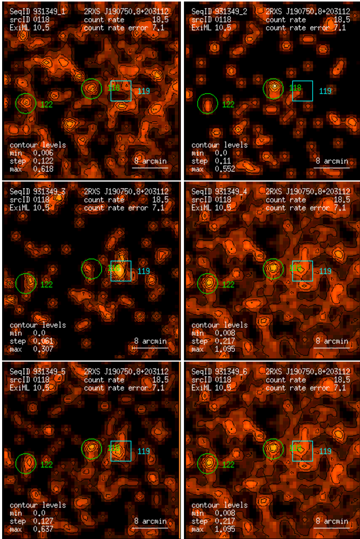
Figure 118: RASS 931349: detection 0118: band rate images, Gaussian filter: (1) PSPC channels 11 – 41, (2) 52 – 90, (3) 91 – 201, (4) 11 – 235, (5) 52 – 201, (6) 11 – 201. Broad band rates in counts/ks. Band rate contour levels in counts/ks/arcmin 2 .
