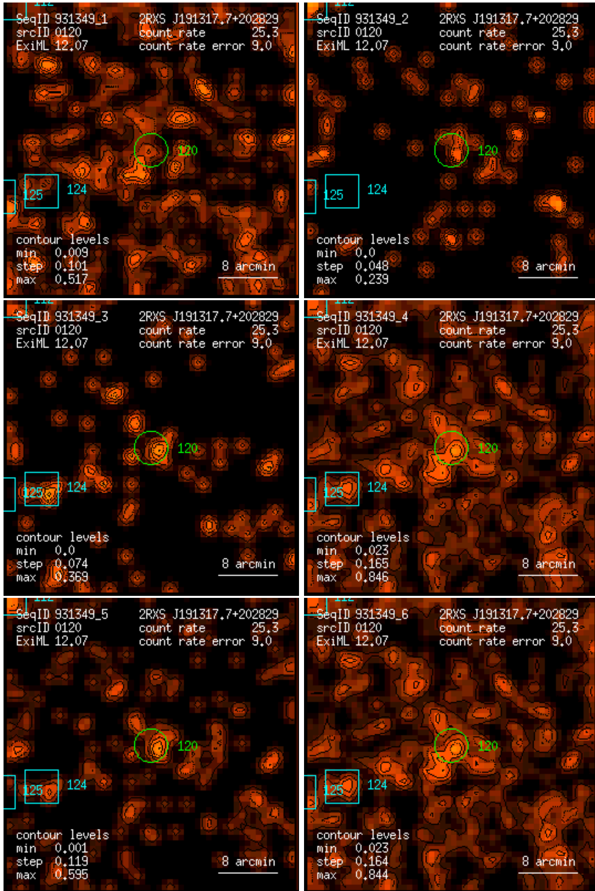
Figure 120: RASS 931349: detection 0120: band rate images, Gaussian filter: (1) PSPC channels 11 – 41, (2) 52 – 90, (3) 91 – 201, (4) 11 – 235, (5) 52 – 201, (6) 11 – 201. Broad band rates in counts/ks. Band rate contour levels in counts/ks/arcmin 2 .
