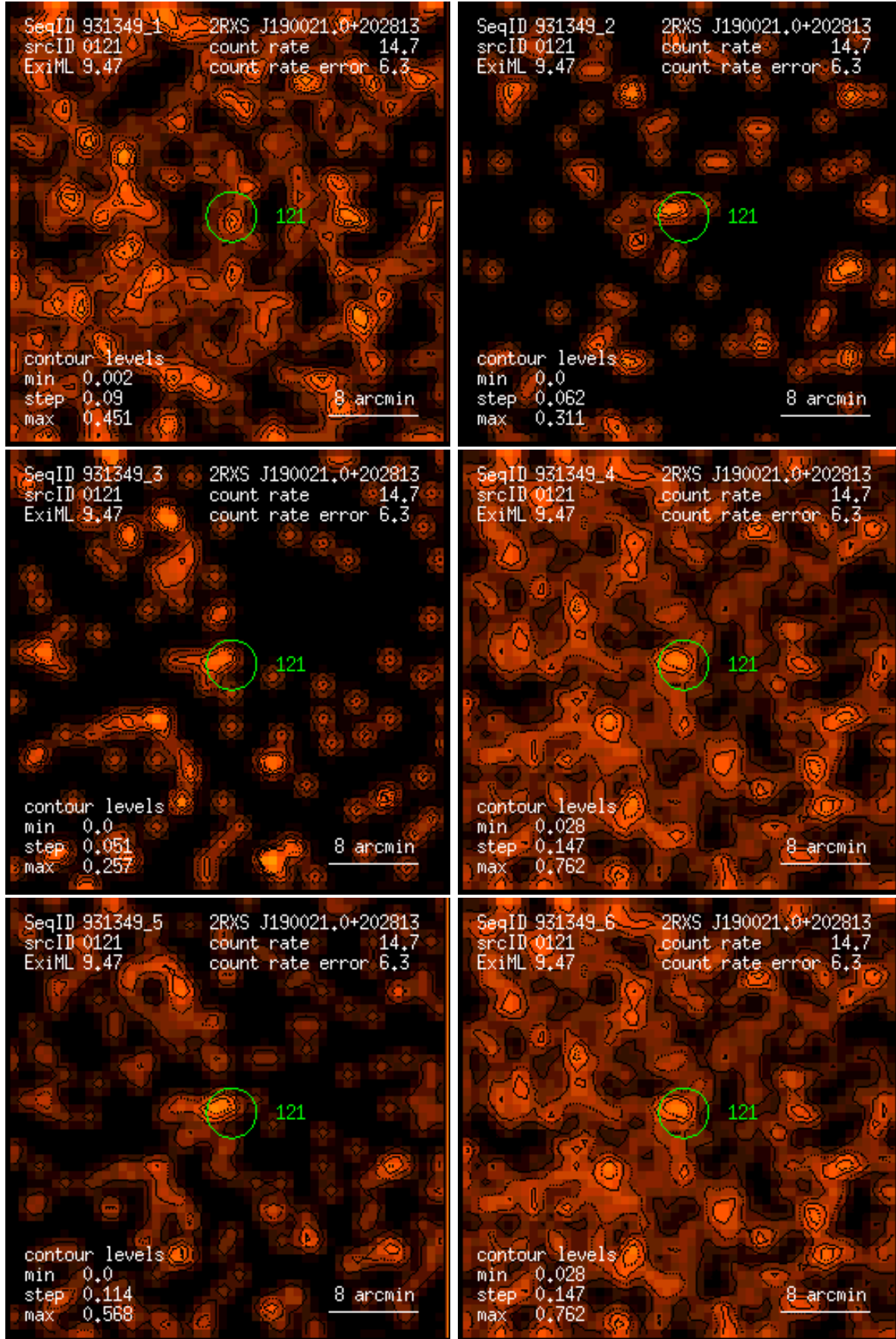
Figure 121: RASS 931349: detection 0121: band rate images, Gaussian filter: (1) PSPC channels 11 – 41, (2) 52 – 90, (3) 91 – 201, (4) 11 – 235, (5) 52 – 201, (6) 11 – 201. Broad band rates in counts/ks. Band rate contour levels in counts/ks/arcmin 2 .
