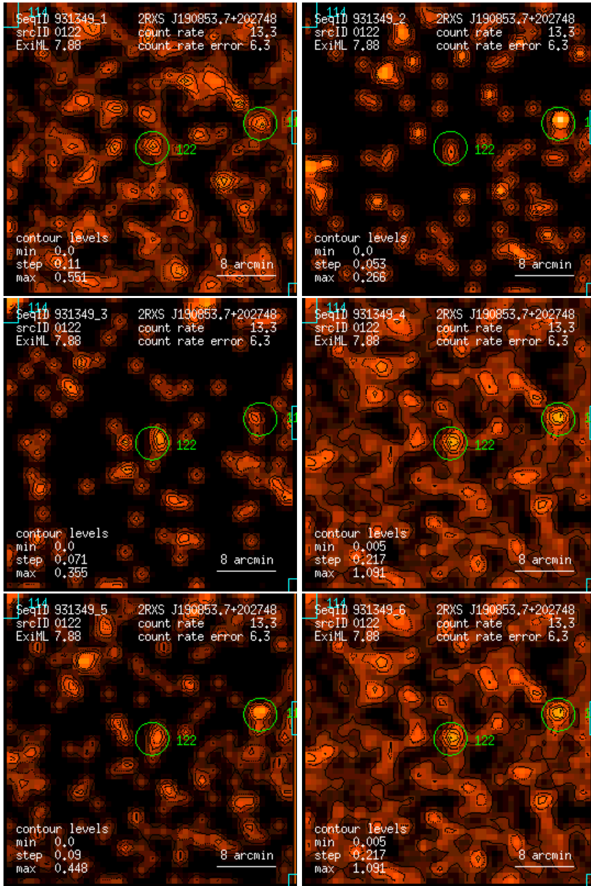
Figure 122: RASS 931349: detection 0122: band rate images, Gaussian filter: (1) PSPC channels 11 – 41, (2) 52 – 90, (3) 91 – 201, (4) 11 – 235, (5) 52 – 201, (6) 11 – 201. Broad band rates in counts/ks. Band rate contour levels in counts/ks/arcmin 2 .
