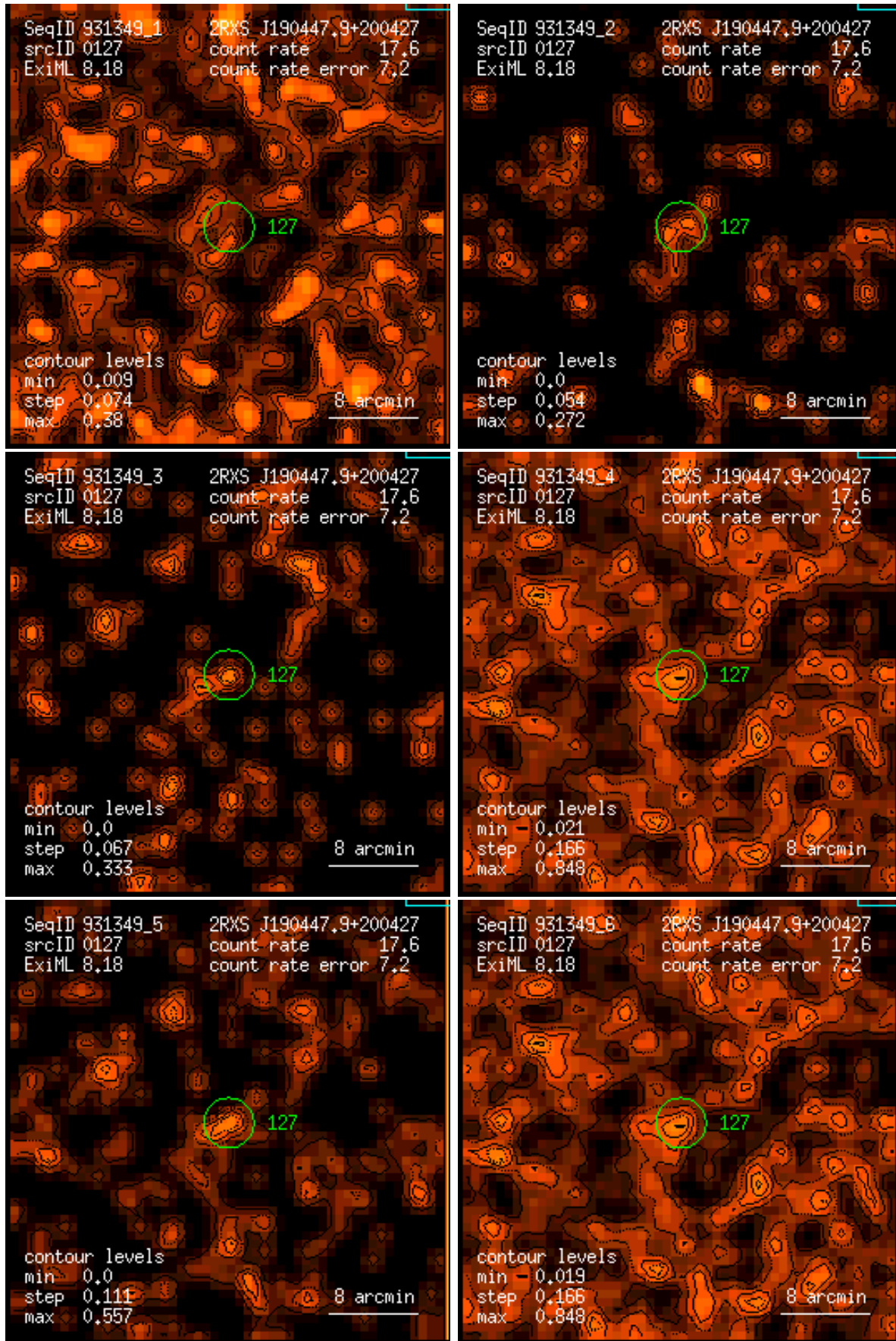
Figure 127: RASS 931349: detection 0127: band rate images, Gaussian filter: (1) PSPC channels 11 – 41, (2) 52 – 90, (3) 91 – 201, (4) 11 – 235, (5) 52 – 201, (6) 11 – 201. Broad band rates in counts/ks. Band rate contour levels in counts/ks/arcmin 2 .
