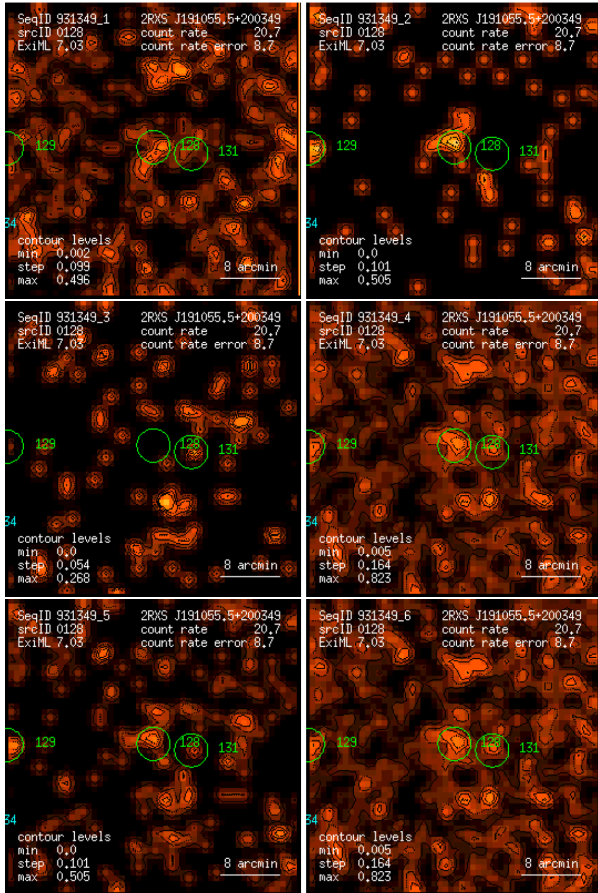
Figure 128: RASS 931349: detection 0128: band rate images, Gaussian filter: (1) PSPC channels 11 – 41, (2) 52 – 90, (3) 91 – 201, (4) 11 – 235, (5) 52 – 201, (6) 11 – 201. Broad band rates in counts/ks. Band rate contour levels in counts/ks/arcmin 2 .
