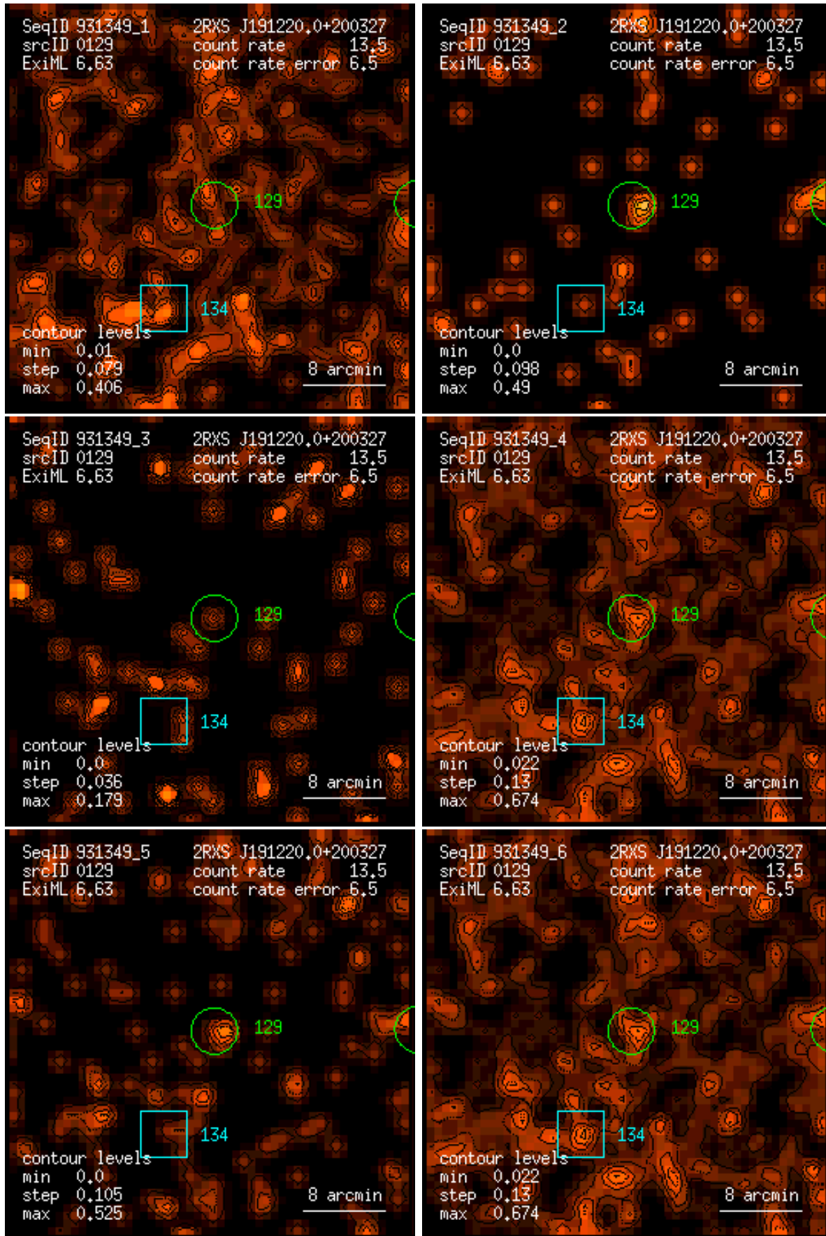
Figure 129: RASS 931349: detection 0129: band rate images, Gaussian filter: (1) PSPC channels 11 – 41, (2) 52 – 90, (3) 91 – 201, (4) 11 – 235, (5) 52 – 201, (6) 11 – 201. Broad band rates in counts/ks. Band rate contour levels in counts/ks/arcmin 2 .
