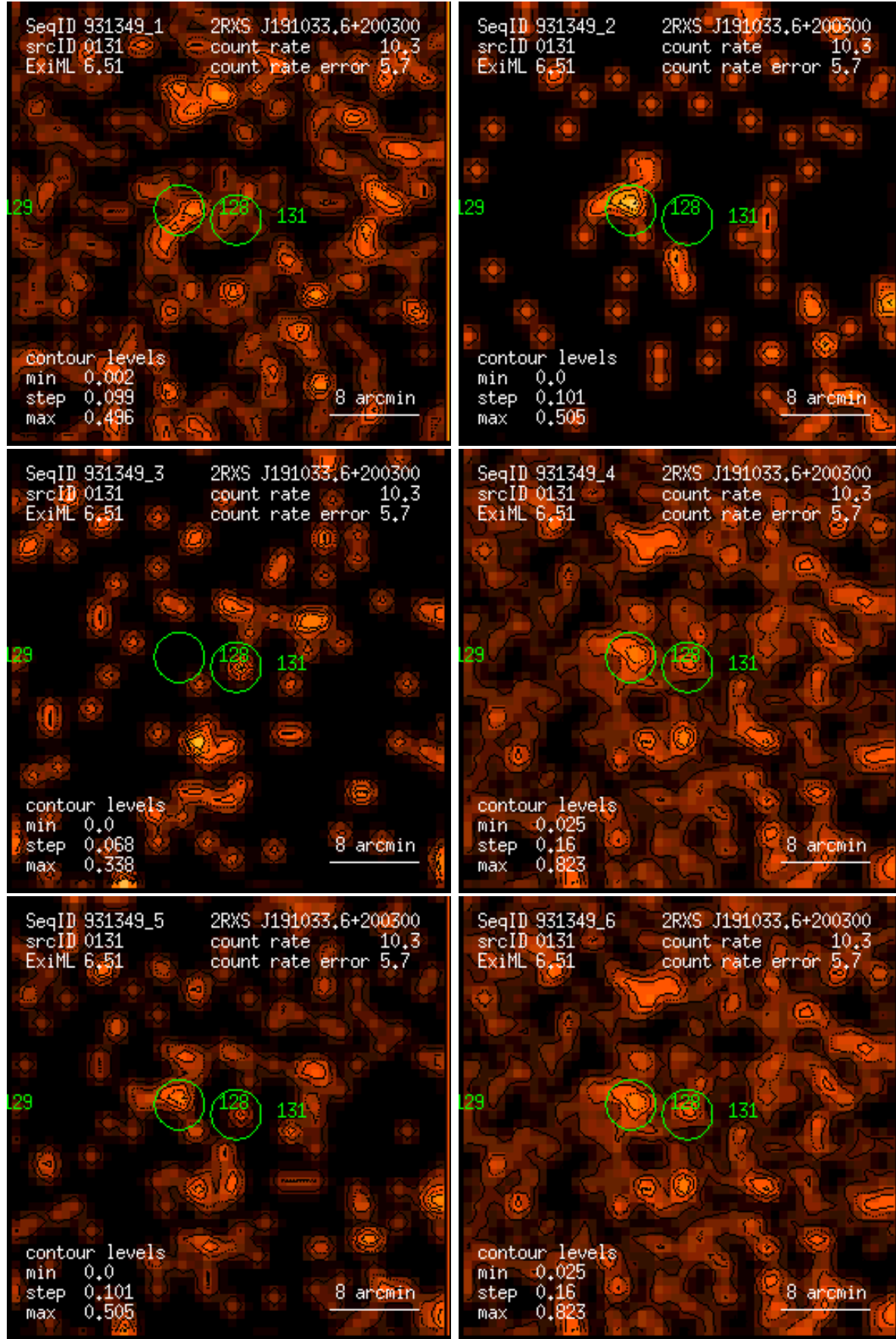
Figure 131: RASS 931349: detection 0131: band rate images, Gaussian filter: (1) PSPC channels 11 – 41, (2) 52 – 90, (3) 91 – 201, (4) 11 – 235, (5) 52 – 201, (6) 11 – 201. Broad band rates in counts/ks. Band rate contour levels in counts/ks/arcmin 2 .
