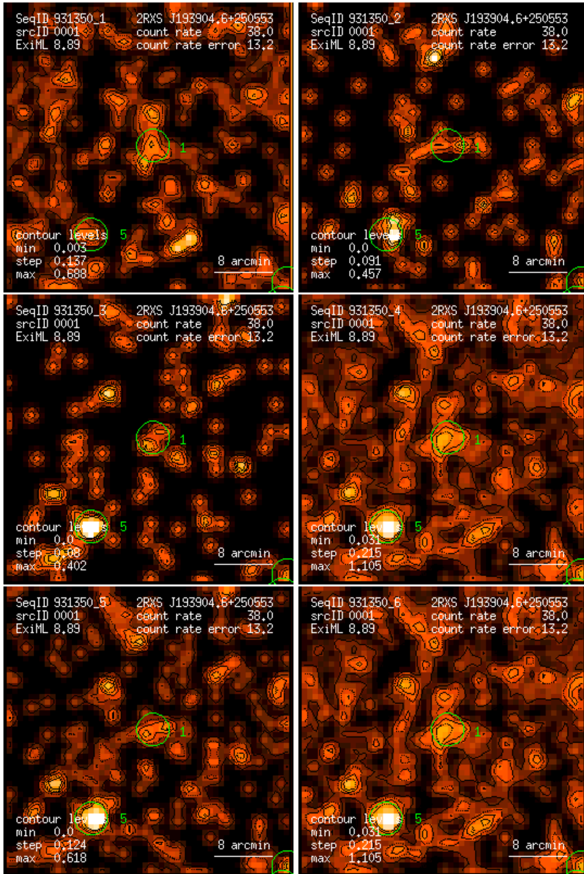
Figure 1: RASS 931350: detection 0001: band rate images, Gaussian filter: (1) PSPC channels 11 – 41, (2) 52 – 90, (3) 91 – 201, (4) 11 – 235, (5) 52 – 201, (6) 11 – 201. Broad band rates in counts/ks. Band rate contour levels in counts/ks/arcmin 2 .
