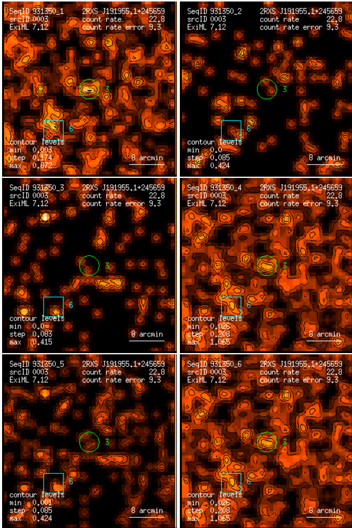
Figure 3: RASS 931350: detection 0003: band rate images, Gaussian filter: (1) PSPC channels 11 – 41, (2) 52 – 90, (3) 91 – 201, (4) 11 – 235, (5) 52 – 201, (6) 11 – 201. Broad band rates in counts/ks. Band rate contour levels in counts/ks/arcmin 2 .
