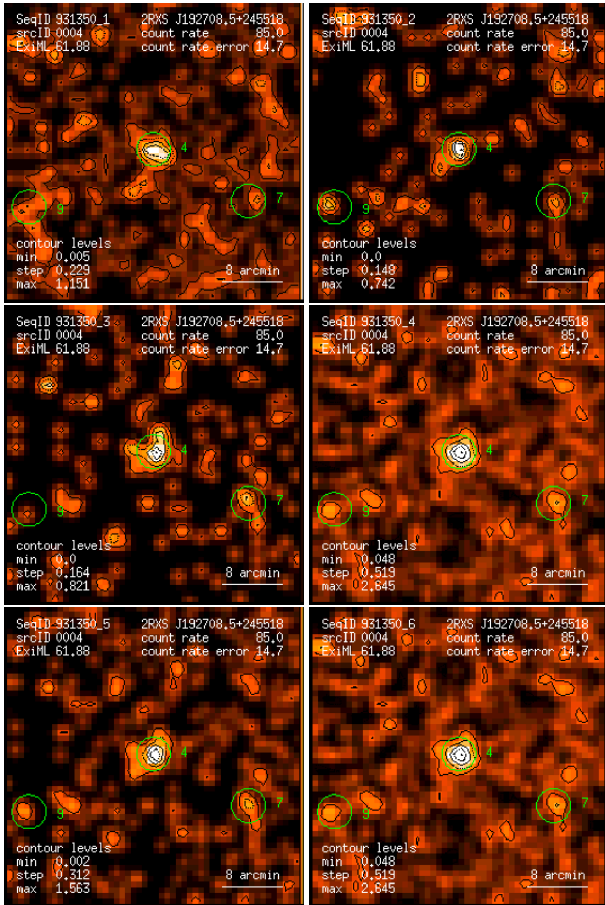
Figure 4: RASS 931350: detection 0004: band rate images, Gaussian filter: (1) PSPC channels 11 – 41, (2) 52 – 90, (3) 91 – 201, (4) 11 – 235, (5) 52 – 201, (6) 11 – 201. Broad band rates in counts/ks. Band rate contour levels in counts/ks/arcmin 2 .
