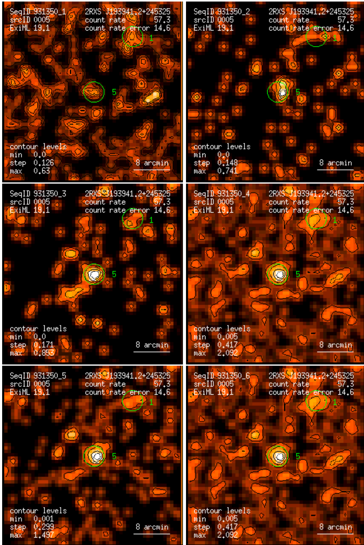
Figure 5: RASS 931350: detection 0005: band rate images, Gaussian filter: (1) PSPC channels 11 – 41, (2) 52 – 90, (3) 91 – 201, (4) 11 – 235, (5) 52 – 201, (6) 11 – 201. Broad band rates in counts/ks. Band rate contour levels in counts/ks/arcmin 2 .
