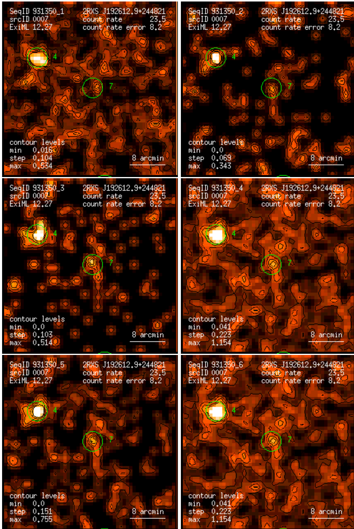
Figure 7: RASS 931350: detection 0007: band rate images, Gaussian filter: (1) PSPC channels 11 – 41, (2) 52 – 90, (3) 91 – 201, (4) 11 – 235, (5) 52 – 201, (6) 11 – 201. Broad band rates in counts/ks. Band rate contour levels in counts/ks/arcmin 2 .
