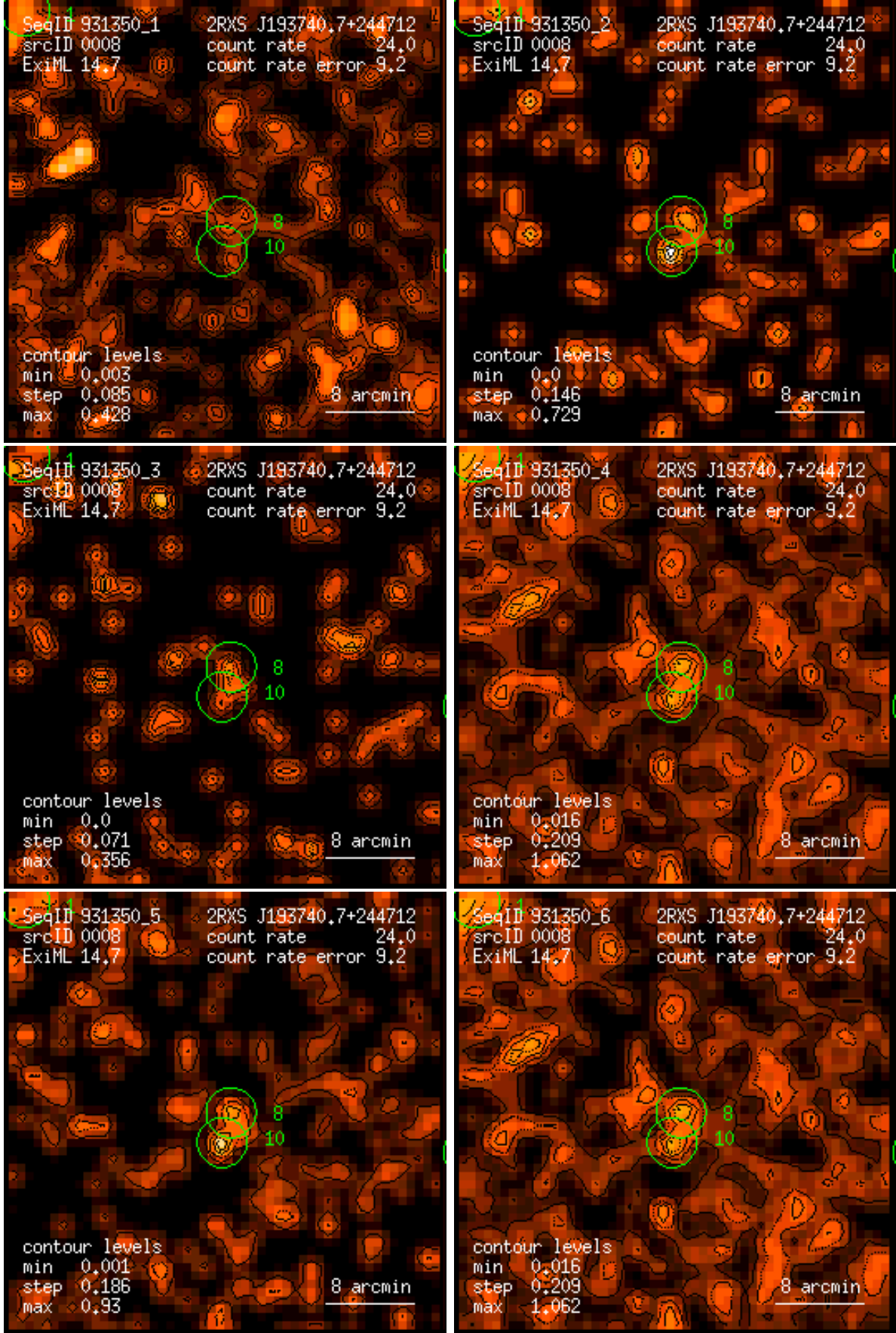
Figure 8: RASS 931350: detection 0008: band rate images, Gaussian filter: (1) PSPC channels 11 – 41, (2) 52 – 90, (3) 91 – 201, (4) 11 – 235, (5) 52 – 201, (6) 11 – 201. Broad band rates in counts/ks. Band rate contour levels in counts/ks/arcmin 2 .
