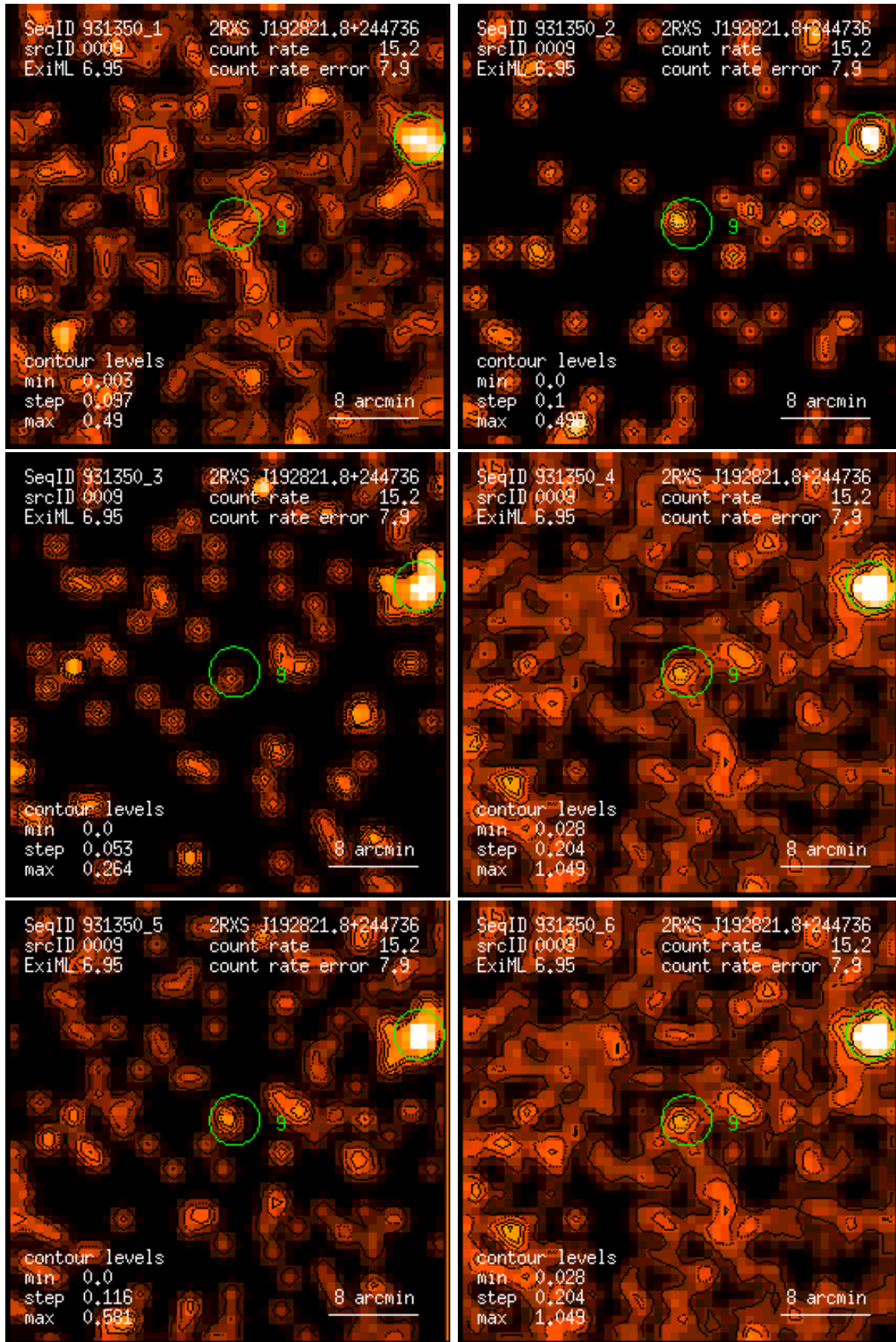
Figure 9: RASS 931350: detection 0009: band rate images, Gaussian filter: (1) PSPC channels 11 – 41, (2) 52 – 90, (3) 91 – 201, (4) 11 – 235, (5) 52 – 201, (6) 11 – 201. Broad band rates in counts/ks. Band rate contour levels in counts/ks/arcmin 2 .
