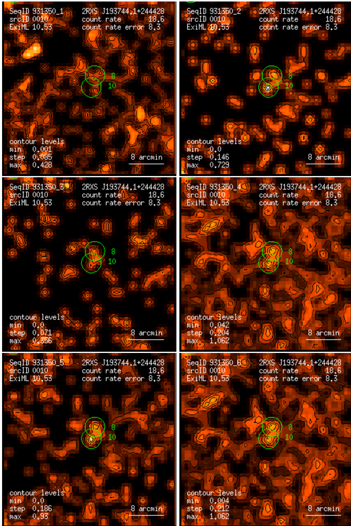
Figure 10: RASS 931350: detection 0010: band rate images, Gaussian filter: (1) PSPC channels 11 – 41, (2) 52 – 90, (3) 91 – 201, (4) 11 – 235, (5) 52 – 201, (6) 11 – 201. Broad band rates in counts/ks. Band rate contour levels in counts/ks/arcmin 2 .
