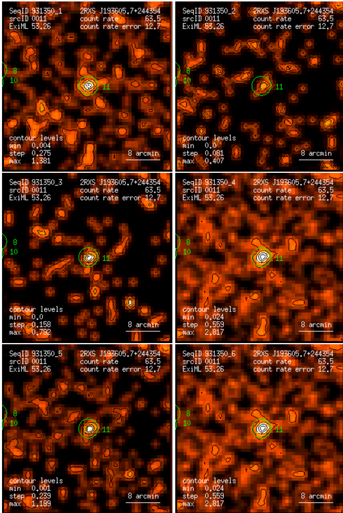
Figure 11: RASS 931350: detection 0011: band rate images, Gaussian filter: (1) PSPC channels 11 – 41, (2) 52 – 90, (3) 91 – 201, (4) 11 – 235, (5) 52 – 201, (6) 11 – 201. Broad band rates in counts/ks. Band rate contour levels in counts/ks/arcmin 2 .
