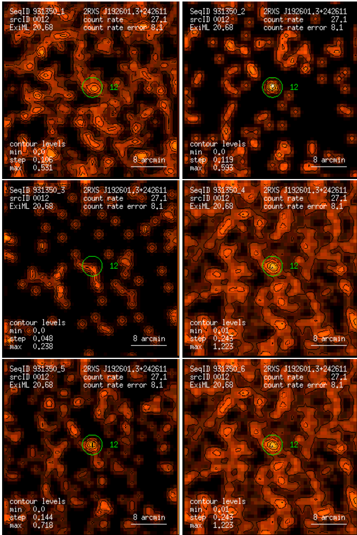
Figure 12: RASS 931350: detection 0012: band rate images, Gaussian filter: (1) PSPC channels 11 – 41, (2) 52 – 90, (3) 91 – 201, (4) 11 – 235, (5) 52 – 201, (6) 11 – 201. Broad band rates in counts/ks. Band rate contour levels in counts/ks/arcmin 2 .
