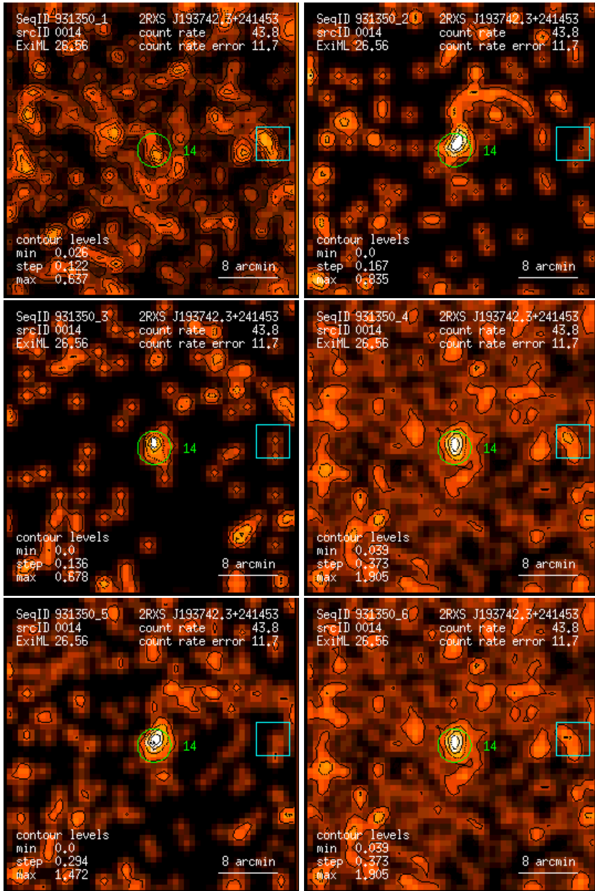
Figure 14: RASS 931350: detection 0014: band rate images, Gaussian filter: (1) PSPC channels 11 – 41, (2) 52 – 90, (3) 91 – 201, (4) 11 – 235, (5) 52 – 201, (6) 11 – 201. Broad band rates in counts/ks. Band rate contour levels in counts/ks/arcmin 2 .
