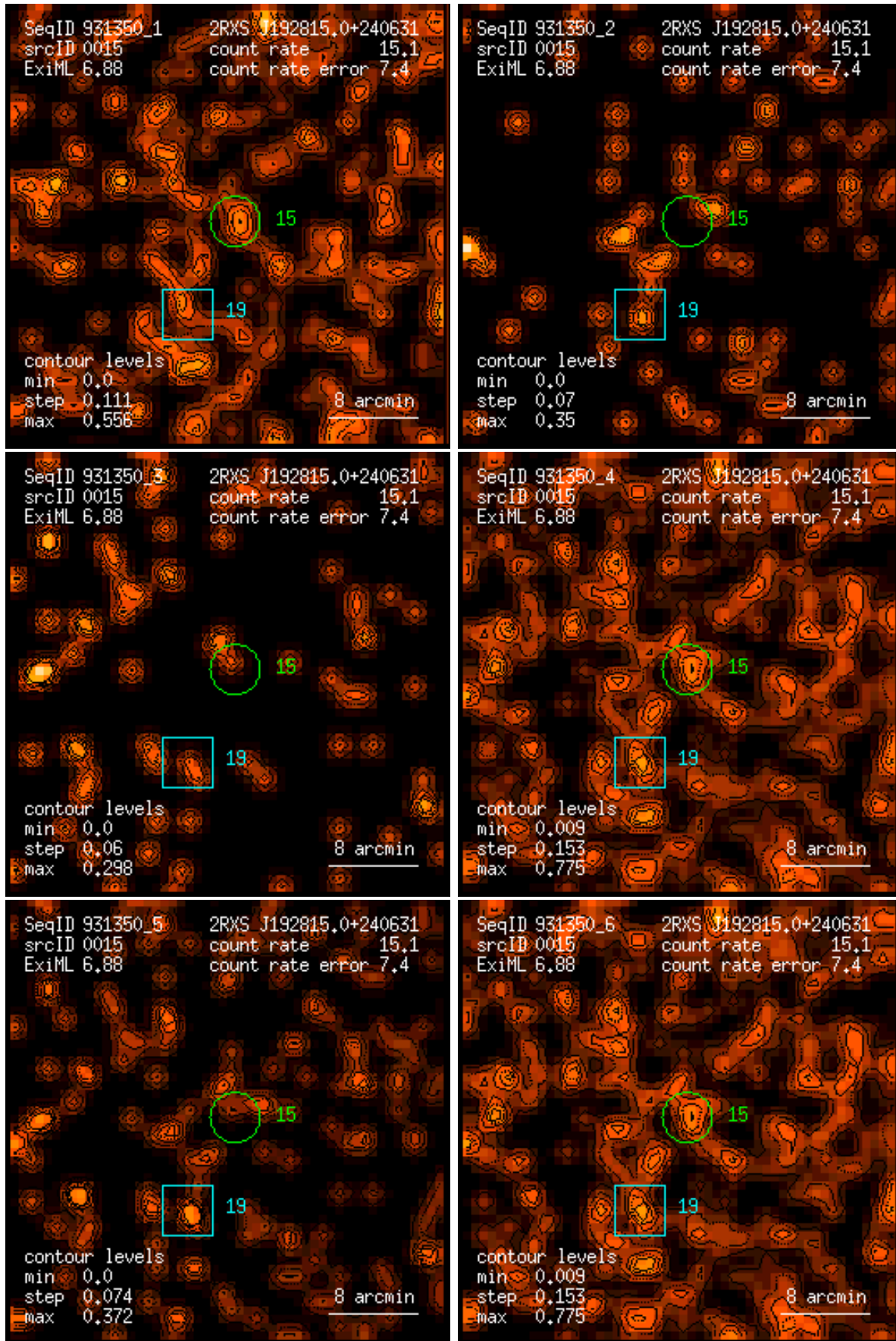
Figure 15: RASS 931350: detection 0015: band rate images, Gaussian filter: (1) PSPC channels 11 – 41, (2) 52 – 90, (3) 91 – 201, (4) 11 – 235, (5) 52 – 201, (6) 11 – 201. Broad band rates in counts/ks. Band rate contour levels in counts/ks/arcmin 2 .
