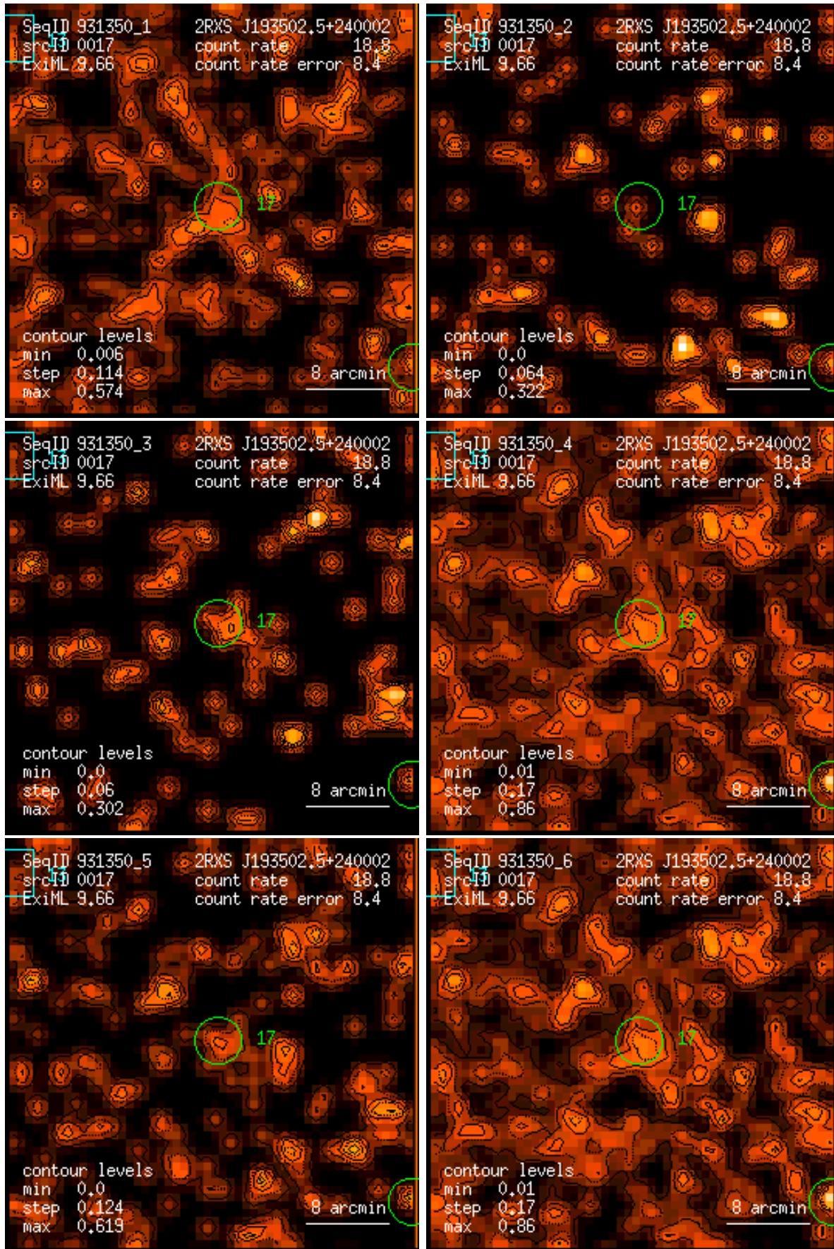
Figure 17: RASS 931350: detection 0017: band rate images, Gaussian filter: (1) PSPC channels 11 – 41, (2) 52 – 90, (3) 91 – 201, (4) 11 – 235, (5) 52 – 201, (6) 11 – 201. Broad band rates in counts/ks. Band rate contour levels in counts/ks/arcmin 2 .
