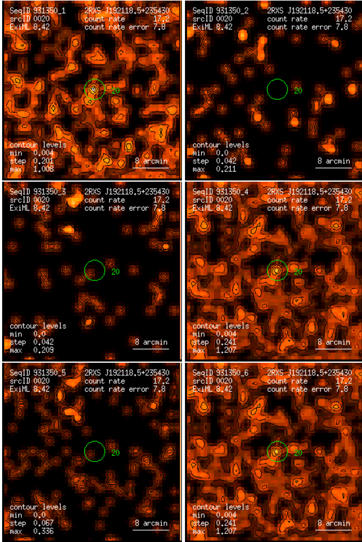
Figure 20: RASS 931350: detection 0020: band rate images, Gaussian filter: (1) PSPC channels 11 – 41, (2) 52 – 90, (3) 91 – 201, (4) 11 – 235, (5) 52 – 201, (6) 11 – 201. Broad band rates in counts/ks. Band rate contour levels in counts/ks/arcmin 2 .
